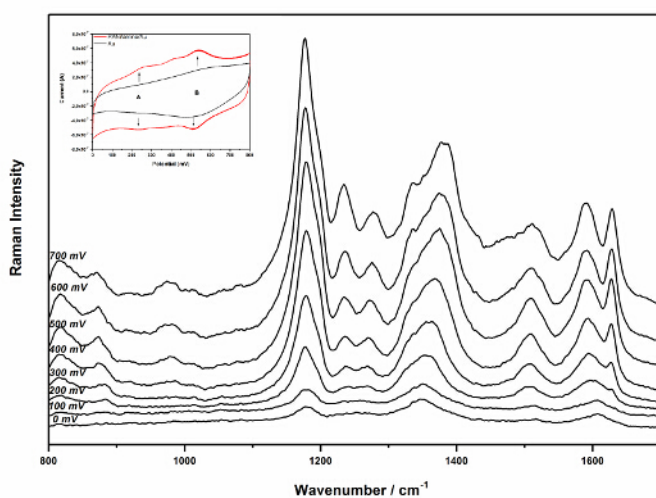
Figure 5: Raman spectra of polyaniline at a different potential; insert: CV curve recorded for the polyaniline film Please click here to view a larger version of this figure.
