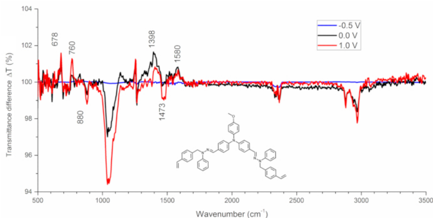
Figure 4: IR spectra of the monomer at various potentials applied Please click here to view a larger version of this figure.
