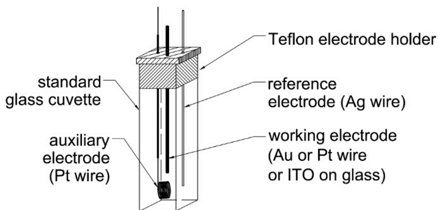
Figure 3: Schemes of Raman spectroelectrochemical cell Please click here to view a larger version of this figure.
