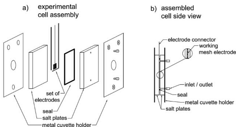
Figure 1: Scheme of transmission IR-spectroelectrochemistry cell (a) and its side view after assembly (b). Please click here to view a larger version of this figure.
