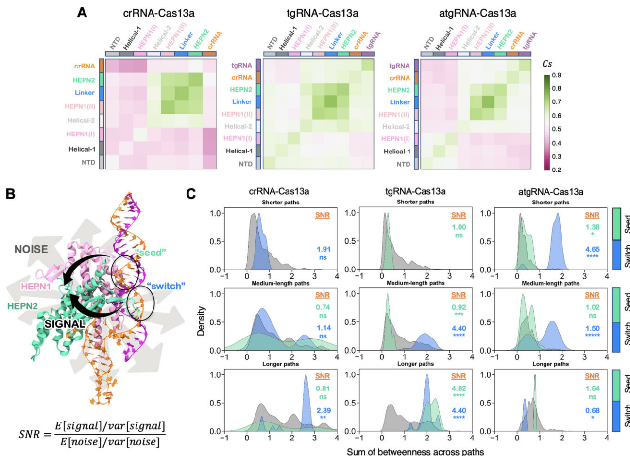
Figure 3. Coupled dynamics and signal-to-noise ratio of communication efficiency. (A) Generalized inter-domain correlation maps for the crRNA-, tgRNA- and atgRNA-bound Cas13a complexes. A pink-to-green colour code is used to describe low-to-high correlations. (B) Schematic representation of the allosteric signals from the crRNA 'seed' (nt. 9–14) and 'switch' (nt. 5–8) regions to the HEPN1-2 catalytic core residues (R472, H1053, H477, R1048) over the noise, computed as the communication between all pairs of crRNA bases and Cas13a residues. Two black arrows are used to indicate the signal standing up over the noise, depicted using grey arrows. The signal-to-noise Ratio (SNR) is computed as the mean-variance ratio ( E[I]/\text{var}[I] ) of the signal over the noise (details in the Material and methods). (C) Distribution of the signals from the crRNA 'seed' (green) and 'switch' (blue) regions to the catalytic core residues, plotted on the background of noise (grey), across short (6–8 edge counts), medium (9–11), and long paths (12–14). The statistical significance of the signals over the noise was computed using Z-score statistics with a two-tailed hypothesis ( P -value reference: not significant, ns P > 0.01 , * P \leq 0.01 , ** P \leq 0.001 , *** P \leq 0.0001 , **** P \leq 0.00001 ). Values of SNR are also reported for each sourcing region.
