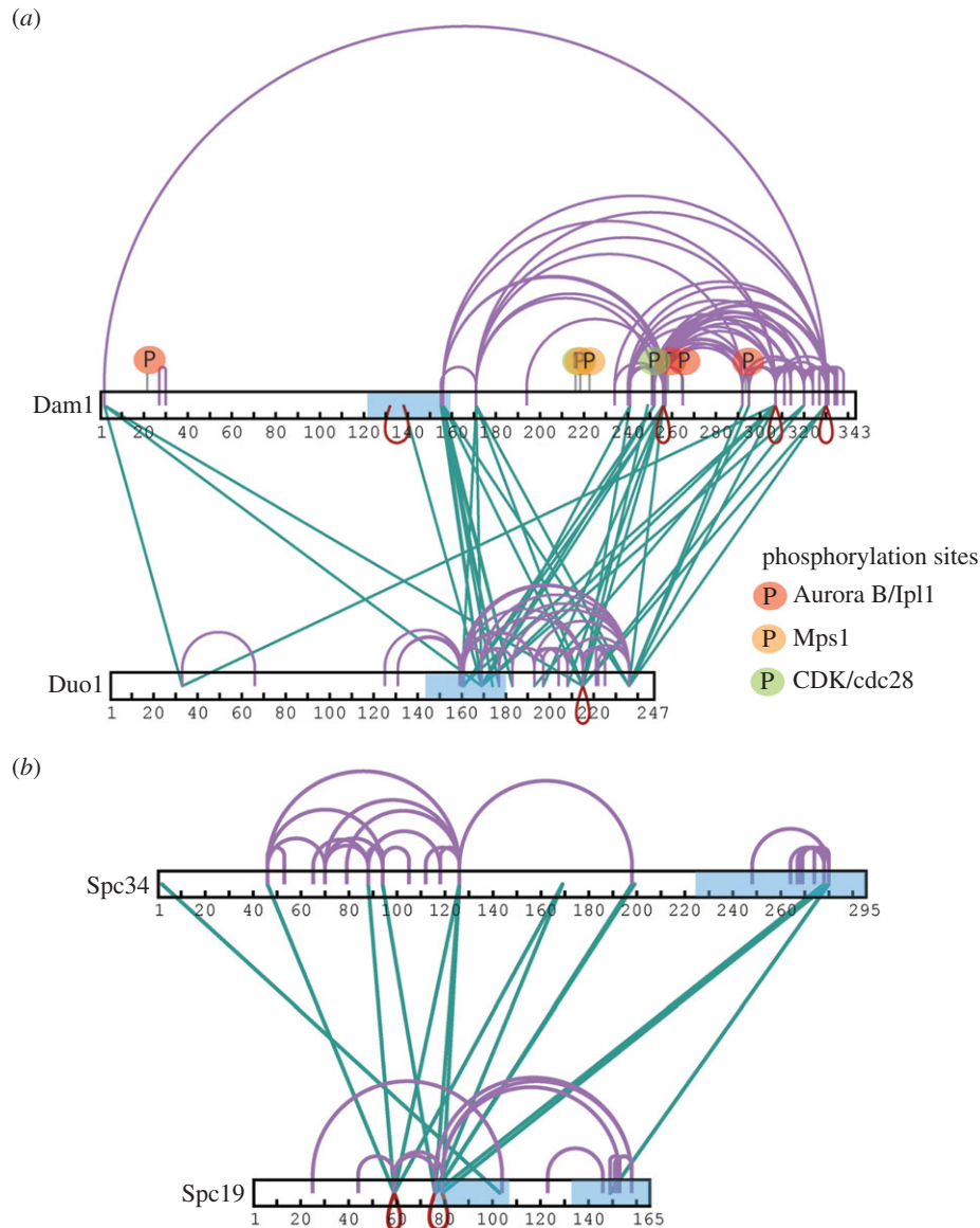
Figure 2. Duo1/Dam1 and Spc34/Spc19 form tight interfaces within the Dam1 complex. Cross-link maps for (a) Duo1 and Dam1 and (b) Spc19 and Spc34 show intramolecular and intermolecular cross-links, isolated from in-solution digestion of the Dam1 complex. Green cross-links represent intermolecular links. Red and purple connections represent intermolecular self-links (between homodimers) and intermolecular or intramolecular self-cross-links, respectively. Predicted coiled coil regions are highlighted in blue. Regulatory sites within Dam1 targeted by Cdc28/CDK1 (S216, S250), Ipl1 (S20, S257, S265, S292) and Mps1 (S218 and S221) are highlighted in green, red and orange, respectively.
