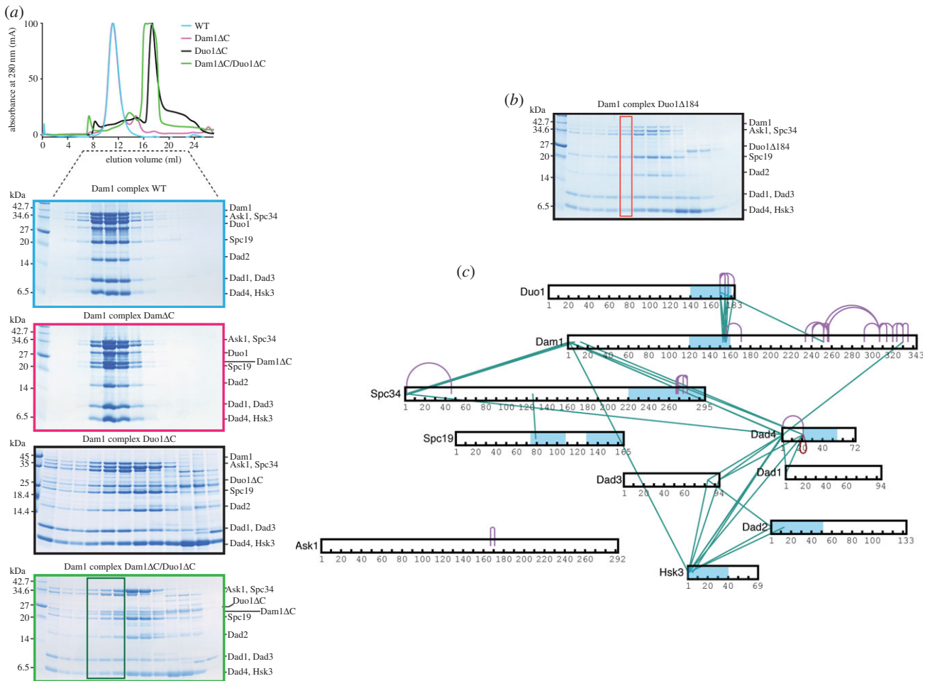
Figure 5. The C terminus of Duo1 is important for the structural integrity of the Dam1 complex. (a) Top, gel filtration elution profile of Dam1 complex (light blue), Dam1 complex Dam1 \Delta C (magenta), Dam1 complex Duo1 \Delta C (black), and Dam1 complex Dam1 \Delta C/Duo1 \Delta C (green). Bottom, protein gels showing the size-exclusion chromatography profile for each Dam1 complex mutant. Fractions boxed in dark green were tested in microtubule co-sedimentation assays in figure 6. (b) Protein gel showing the size-exclusion chromatography profile for the Dam1 complex Duo1 \Delta 184. The fraction boxed in red was used for cross-linking and mass spectrometry analysis in (c). (c) Cross-links within the Dam1 complex Duo1 \Delta 184 in the presence of BS3. Predicted coiled coil regions are in blue.
