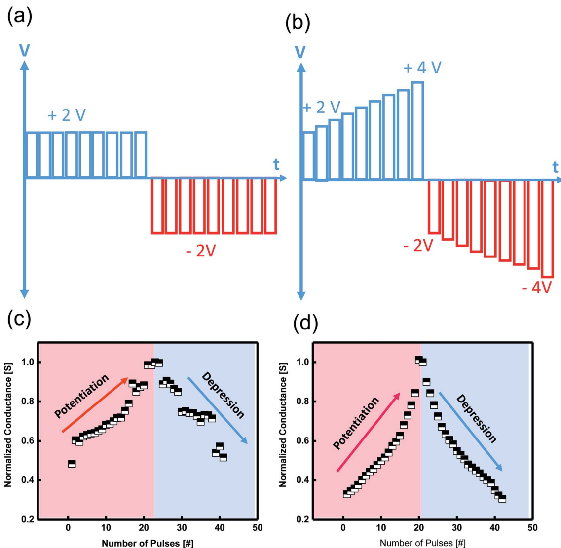
Fig. 6 Various programming pulse schemes. (a) Successive identical and (b) non-identical neuron spikes. (c and d) Normalized potentiation and depression properties of TaO 2-x thin-film memristor with two different pulse schemes. The non-identical spikes lead to a linear synaptic behavior with a slope of 1. Using nonidentical presynaptic spikes, a significant improvement in symmetry was observed.
