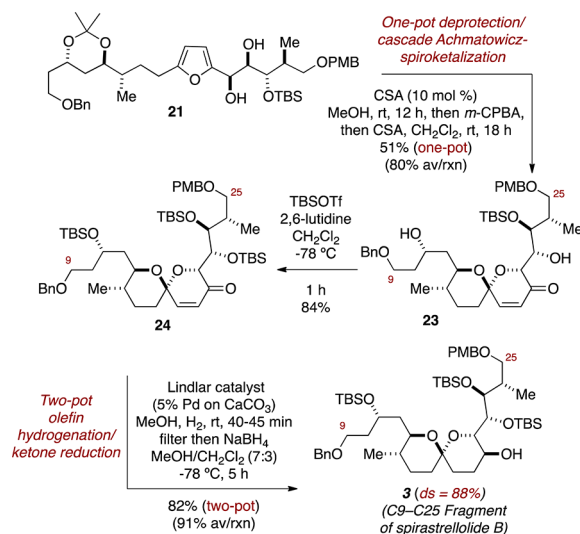
Scheme 5. Alternative Synthesis of the C9–C25 Fragment
