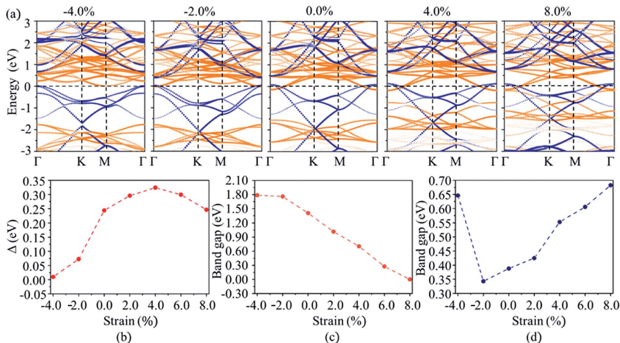
Fig. 5 (a) The projected band structures of MoS_2/C_3N heterojunction with strain applied. The blue dots and orange dots represents the band contributions from C_3N and MoS_2 , respectively. Evolution of the (b) band overlap, band gap of (c) MoS_2 and (d) C_3N as a function of strain.
