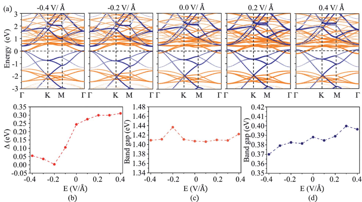
Fig. 4 (a) The projected band structures of MoS_2/C_3N heterojunction with electric field applied. The blue dots and orange dots represent the band contributions from C_3N and MoS_2 , respectively. Evolution of the (b) band overlap, band gap of (c) MoS_2 and (d) C_3N as a function of the external electric field.
