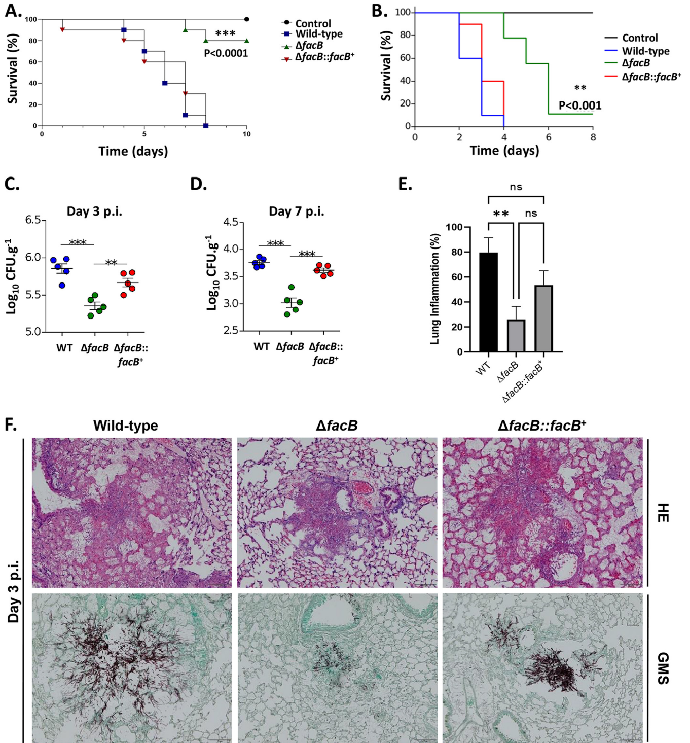
FIG 6 FacB is crucial for virulence in both insect and murine models of invasive aspergillosis. (A and B) Survival curves ( n=10/\text{strain} and n=5 for control) of Galleria mellonella (A) and mice (B) infected with the respective A. fumigatus strains. Phosphate-buffered saline (PBS) without conidia was given as a negative control. The indicated P values are based on the log rank, Mantel-Cox, and Gehan-Breslow-Wilcoxon tests comparing the facB deletion strain to the WT and facB complemented strains. (C and D) Fungal burden in murine lungs after 3 (C) and 7 (D) days postinfection (p.i.) with the different A. fumigatus strains. Murine lungs were excised, ruptured, and resuspended, before dilutions were prepared that were incubated on plates containing complete medium. Fungal growth was assessed by counting the CFU on the plates for each dilution. (E) Inflammation in murine lungs after 3 days postinfection (p.i.) with the different A. fumigatus strains. Murine lungs were excised, and slides of lung sections were prepared. To quantify lung inflammation of infected animals, inflamed areas on slide images were analyzed using the thresholding tool in ImageJ software. Values are averages \pm standard deviations (error bars) of three biological replicates (lungs from different mice). Values that are significantly different in a two-way multiple comparison ANOVA test are indicated as follows: *, P value < 0.01 ; **, P value < 0.001 ; ***, P value < 0.0001 . (G) Histopathology of mice infected with the different A. fumigatus strains. Lungs were excised at 3 days postinfection (p.i.) before lung sections were prepared and stained with HE (hematoxylin and eosin) or with Grocott's methenamine silver (GMS).
