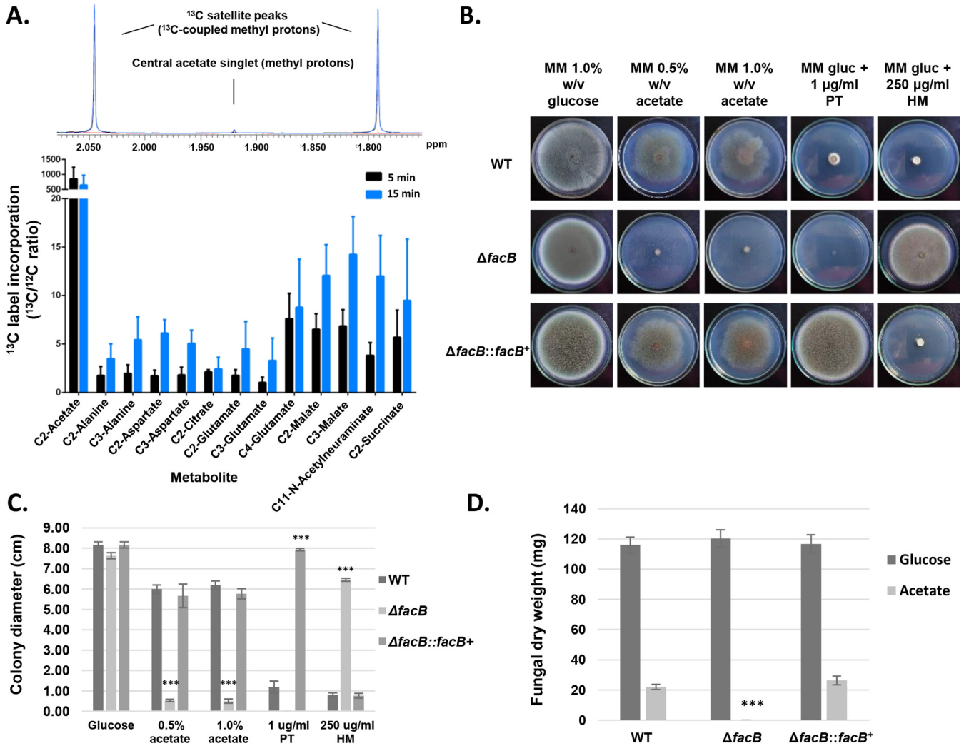
FIG 1 Acetate metabolism in A. fumigatus . (A) One- and two-dimensional (1D and 2D) NMR (nuclear magnetic resonance) analysis of 13 C 2 -labeled acetate incorporation and metabolism. (Top) Expansion of 1D 1 H NMR spectra of fungal cell extracts showing the increase in acetate carbon satellite peaks upon culture of A. fumigatus in 13 C 2 -acetate-containing medium. (Bottom) 13 C/ 12 C ratios for metabolites that incorporated 13 C derived from acetate, as determined through integration of 1 H- 13 C HSQC (heteronuclear single quantum coherence) spectra recorded for extracts of fungal cells grown for 5 and 15 min in medium containing [ 13 C 2 ]acetate in comparison to nonlabeled control cultures. Values are averages plus standard deviations (error bars) of biological triplicates. (B to D) The transcription factor FacB is essential for growth in the presence of acetate. Strains were grown for 5 days (B and C) or 3 days (D) in either solid (B and C) or liquid (D) minimal medium (MM) supplemented with 1% (wt/vol) glucose (gluc) (B and D), 0.5% (wt/vol) (B) or 1% (wt/vol) (B and D) acetate before radial diameter (C) or fungal dry weight (D) was measured. To ensure homologous integration of facB in the complementation strain, strains were grown in the presence of pyrithiamine (PT) ( facB was reintroduced into the \Delta facB strain using the PT-resistant marker gene) and hygromycin (HM) ( facB was deleted using the HM resistance marker gene) (B and C). Plate pictures (B) are representative for the average radial diameter shown in panel C. Values are averages \pm standard deviations (error bars) of biological triplicates. The values for the facB deletion strain are significantly different from the values for the wild-type (WT) strain in a two-way multiple comparison analysis of variance (ANOVA) test as indicated: ***, P value of <0.0001.
