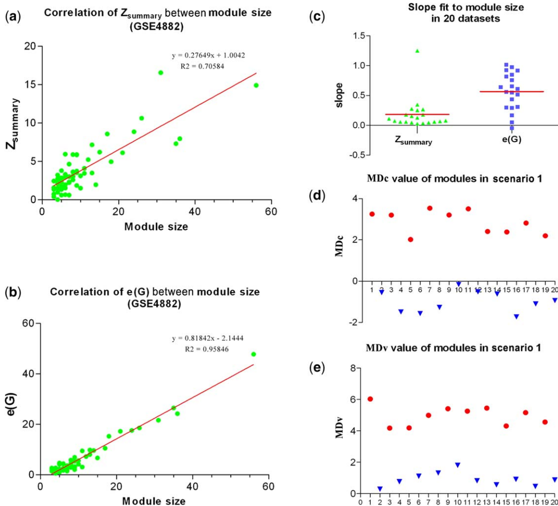
Figure 1 (a,b) Correlation between Z_{\text{summary}} / e(G) (y-axis) and module size (x-axis) using GSE4882 as an example. (c) The slope fit value (y-axis) between Z_{\text{summary}} / e(G) and module size in 20 datasets. The red line represents their mean value. (d,e) The conserved Modudaism (MDc)/varied Modudaism (MDv) values of the predefined preserved modules (in red circle) or discrepant modules (in blue triangle) in simulation scenario 1.
