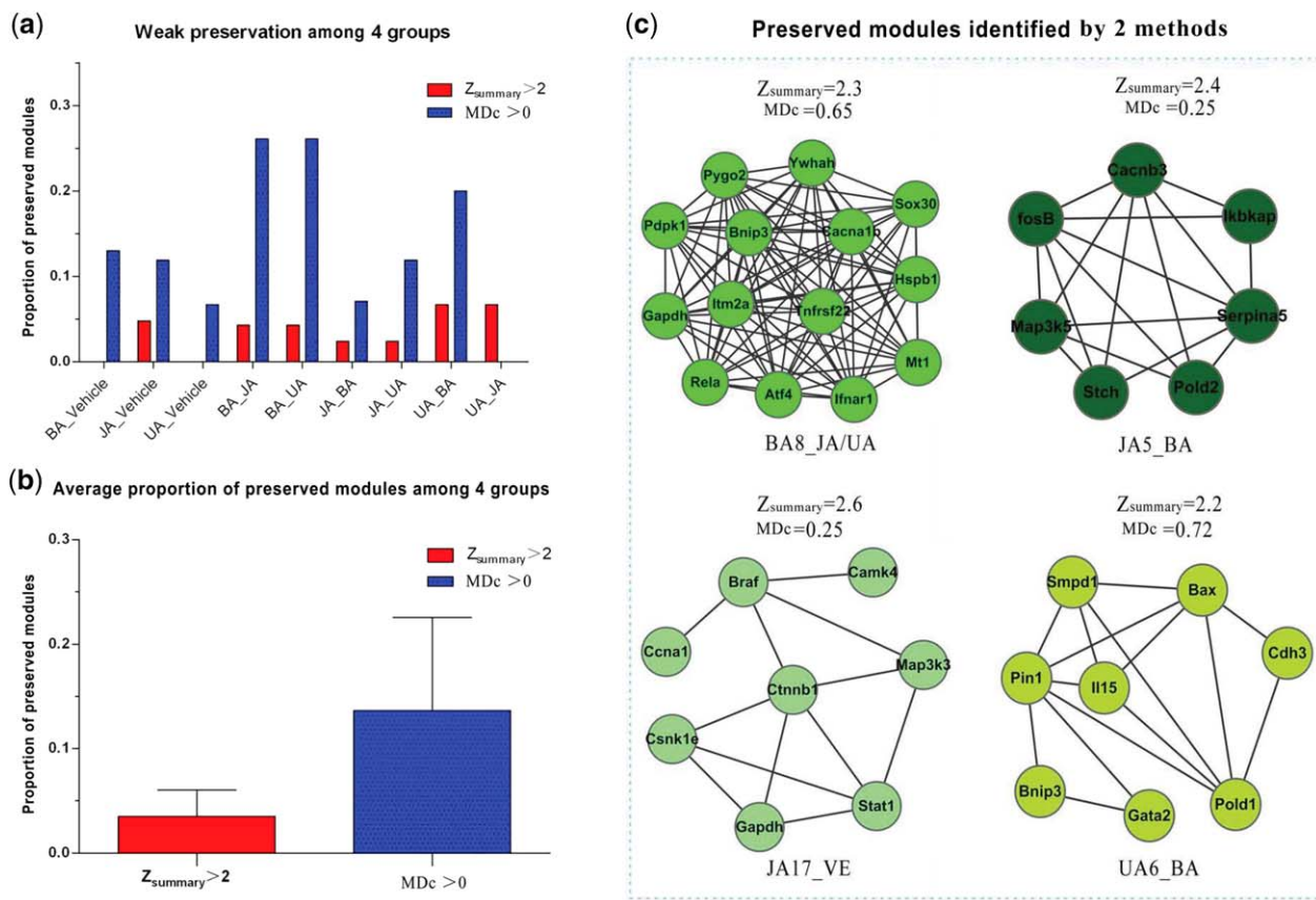
Figure 3 (a) Comparison of the proportions of conserved allosteric modules (CAMs; Z_{summary} \geq 2 or conserved Modudaism ( MDc > 0 )) among baicalin (BA), jasminoidin (JA), ursodeoxycholic acid (UA), and vehicle (VE) groups. (b) The average proportions of CAMs identified by Z_{summary} and MDc in BA, JA, UA, and vehicle groups. (c) The CAMs identified by both Z_{summary} and MDc .
