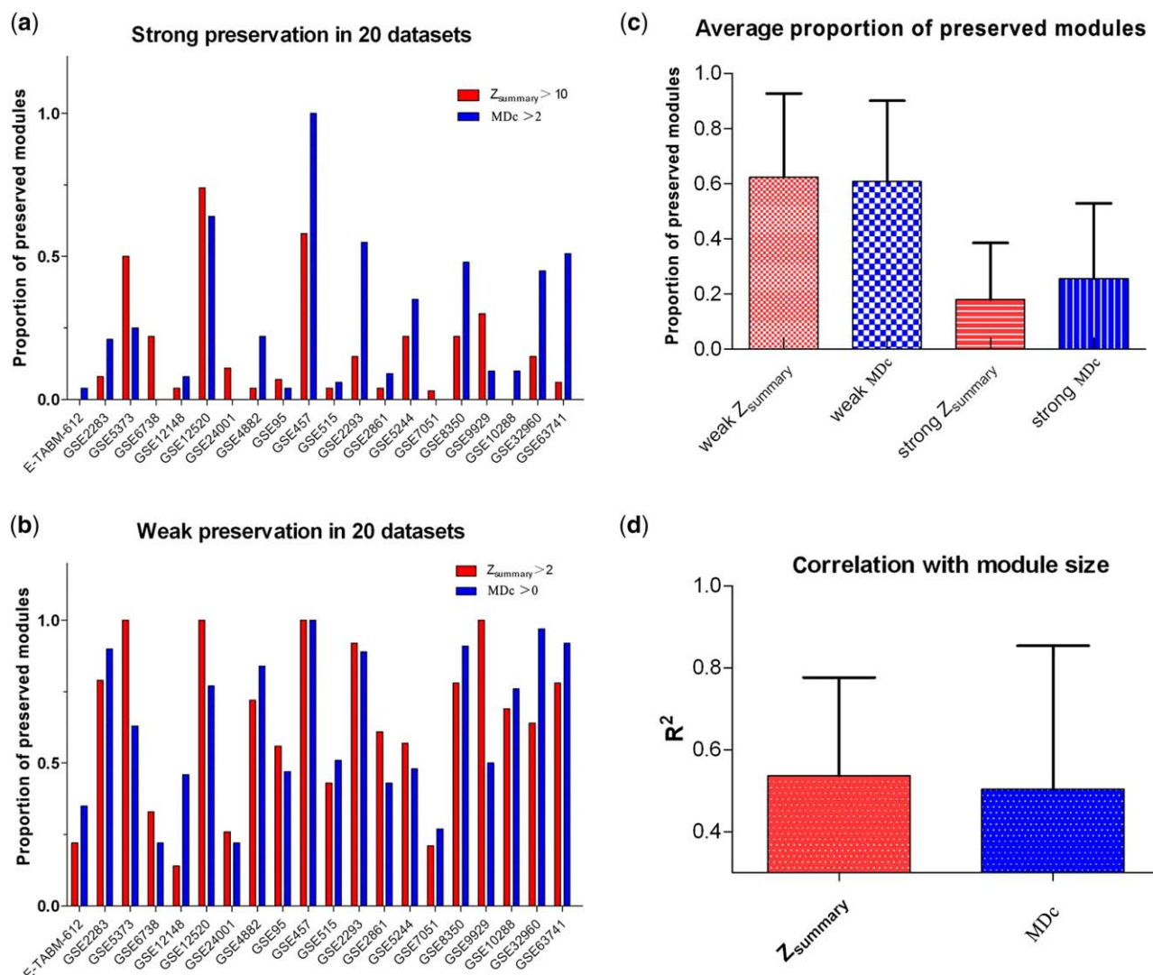
Figure 2 (a,b) Comparison of the proportions of strong preserved modules ( Z_{summary} \geq 10 , conserved Modudaoism (MDc) \geq 2 ) and weak preserved modules ( Z_{summary} \geq 2 , MDc > 0 ) in 20 datasets. (c) The average proportions of strong and weak preserved modules identified by Z_{summary} and MDc in 20 datasets. (d) The correlation coefficient R^2 between Z_{summary}/MDc and module size in 20 datasets.
