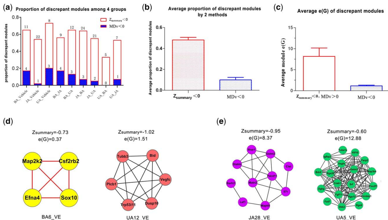
Figure 5 (a) Comparison of the proportions of differential modules ( Z_{summary} < 0 or varied Modudaism (MDv) < 0) among baicalin (BA), jasminoidin (JA), ursodeoxycholic acid (UA) and vehicle (VE) groups. (b) The average proportions of differential modules identified by Z_{summary} and MDv in the four groups. (c) The average e(G) of differential modules in the four groups. (d) The sample on-modules with negative MDv and Z_{summary} values as well as a small e(G) . (e) The sample modules with a negative Z_{summary} value but a large e(G) , which were not identified as on-modules.
