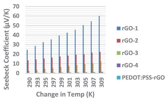
Fig. 8 Effect of temperature gradient on thermoelectric performance of as coated substrate with different weight percent of rGO and PEDOT:PSS nano composite.
