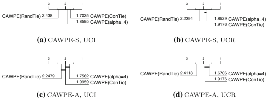
Fig. 15 Critical difference diagrams over test error of CAWPE on the UCI and UCR archives as it stands ( \alpha = 4 ), and against two tuning schemes for the alpha parameter: resolving ties in error estimates randomly (RandTie); and conservatively picking the lowest alpha amongst the ties (ConTie)
