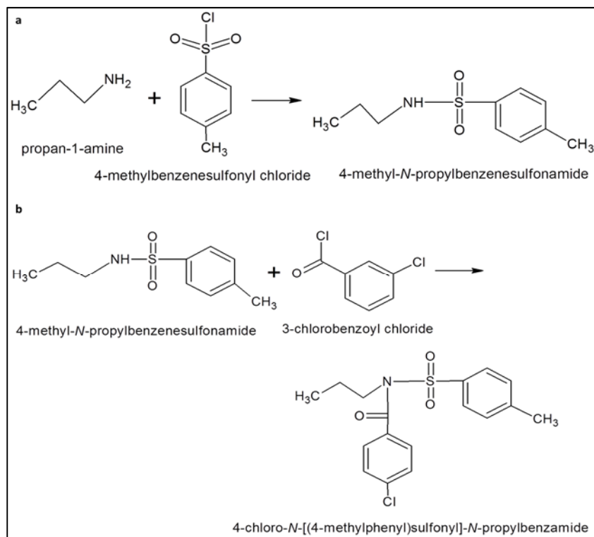
Figure 2: (a) Reaction of propan-1-amine with 4-methylbenzenesulfonyl chloride to produce 4-methyl-N-propylbenzenesulfonamide, (b) 4-methyl-N-propylbenzenesulfonamide was further reacted with 3-chlorobenzoyl chloride to obtain 4-chloro-N-[(4-methylphenyl)sulfonyl]-N-propylbenzamide.
