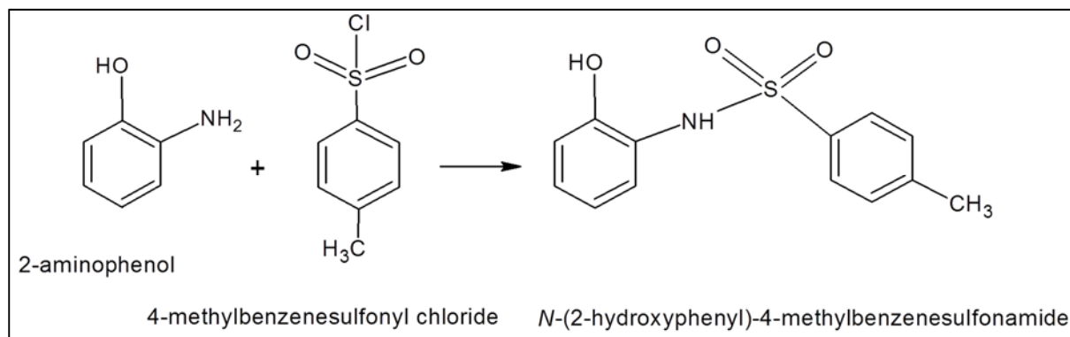
Figure 3: Reaction of 2-aminophenol with 4-methylbenzenesulfonyl chloride producing N-(2-hydroxyphenyl)-4-methyl benzenesulfonamide (1B).
