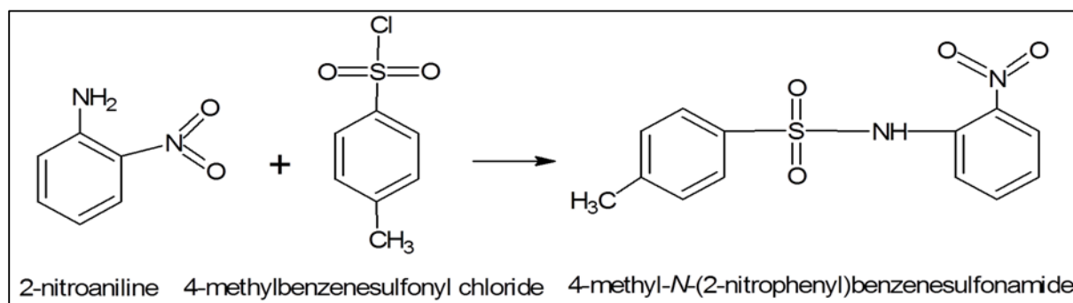
Figure 4: 2-nitroaniline was reacting with 4-methylbenzenesulfonyl chloride to synthesize 4-methyl-N-(2-nitrophenyl) benzenesulfonamide, 1C.
