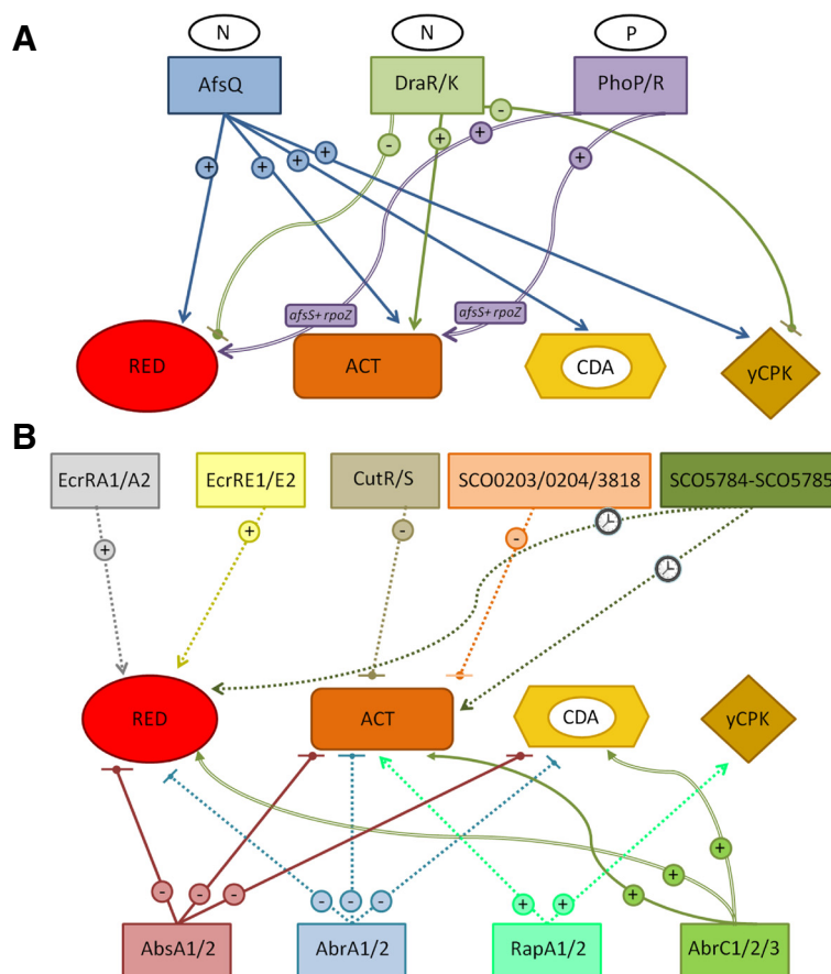
Figure 2 Schematic overview of the regulation of antibiotic production by the TCSs described in this review. A) TCSs with a known signal (Nitrogen, N, or phosphate, P). B) TCSs with an unknown signal. (+) Indicates positive regulation; (-) indicates negative regulation. Straight arrows indicate that the regulation is exerted through the CSRs. A double-lined arrow indicates that regulation is exerted indirectly, and not through CSRs. The intermediate targets of the indirect regulation are shown, in a box within the arrows, when known. A discontinuous line indicates that the regulation mechanism has not yet been studied. The clock indicates timing control in antibiotic biosynthesis.
