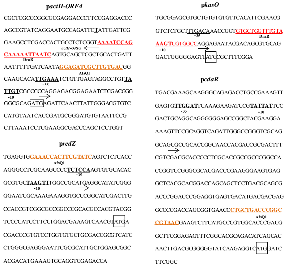
Figure 1 Location of the binding sequences for the S. coelicolor response regulators AfsQ1, DraR in the promoter regions of antibiotic cluster-situated regulators: actII-ORF4 , redZ , kasO , and cdaR [23,24]. Transcription starting points are indicated with an arrow. -10 and -35 sites and translation start codon are also shown.
