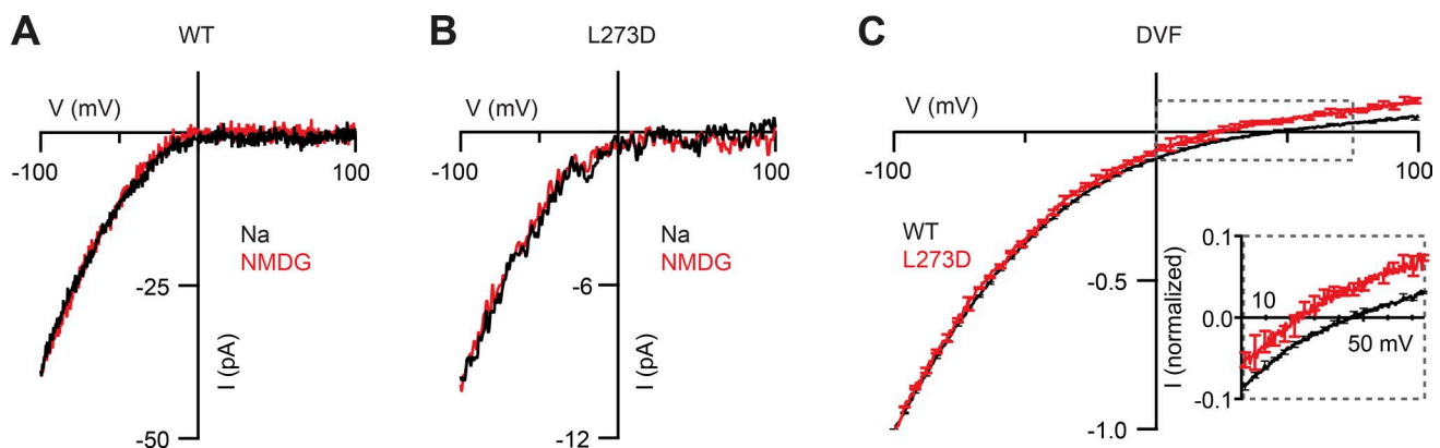
Figure 5. Ion selectivity of L273D currents. I-V relations of hexameric WT and 1xL273D channels in cells coexpressing mCherry-STIM1. Selectivity in physiological Ca 2+ was assessed in 2 mM Ca 2+ Ringer's, in the presence of extracellular Na + (black) or after replacement of Na + by NMDG (red). Exemplar I-V relations of a cell coexpressing mCherry-STIM1 with WT (A) or 1xL273D (B) hexamer channels. No change was observed when extracellular Na + was removed, indicating that Na + does not permeate either WT or 1xL273D channels. (C) I-V relations in DVF Ringer's from WT (black) or 1xL273D (red) channels were normalized to their peak current at -100 mV and averaged (n = 3–4 cells per variant). The SEM is plotted for every 10th point. E rev was reduced in 1xL273D cells (25.9 ± 2.0 mV compared with 45.8 ± 1.2 mV in WT cells; see inset), indicating an increased Cs + to Na + permeability. The average I-V relation for WT Orai1 hexamer is reproduced from Yen et al. (2016) for comparison.
