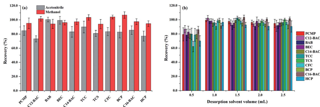
Fig. 5 Effect of (a) desorption solvent type and (b) desorption solvent volume on desorption efficiency of \text{Fe}_3\text{O}_4@PPy .
