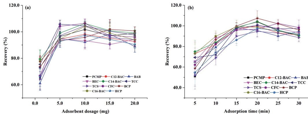
Fig. 4 Effect of (a) adsorbent dosage and (b) adsorption time on extraction efficiency of \text{Fe}_3\text{O}_4@PPy .
