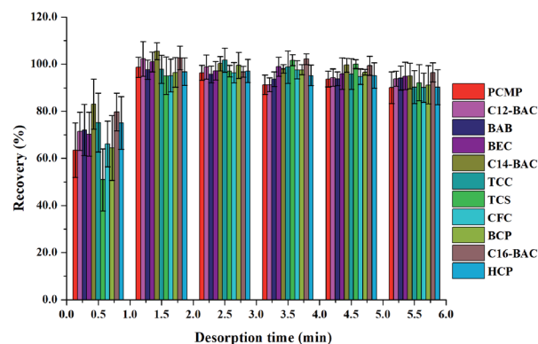
Fig. 6 Effect of desorption time on desorption efficiency of \text{Fe}_3\text{O}_4@PPy .
