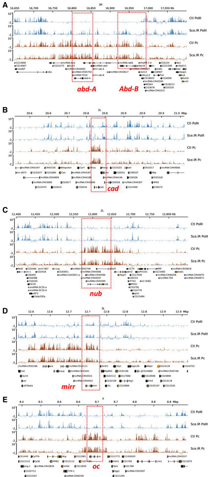
Figure 2 Sce.IR derepression loci are also Dam-Pc binding sites. (A-E) Genome browser views of major de-repression loci. Traces show fold-change of Dam-Pol II fusion over Dam alone, and Dam-Pc fusion over Dam alone for control discs and Ubx > Sce.IR discs. The bithorax region encompassing abd-A and Abd-B (A) is markedly derepressed in Sce.IR discs. These regions also show clear binding of Dam-Pc indicating that they are regions of PcG repression. Note that Ubx expression is unaffected by loss of Sce . Similarly, loci for caudal (B), nubbin (C), mirror (D) and ocelliless (E) show varying degrees of increased Dam-Pol II binding but are all clearly regions of Dam-Pc binding.
