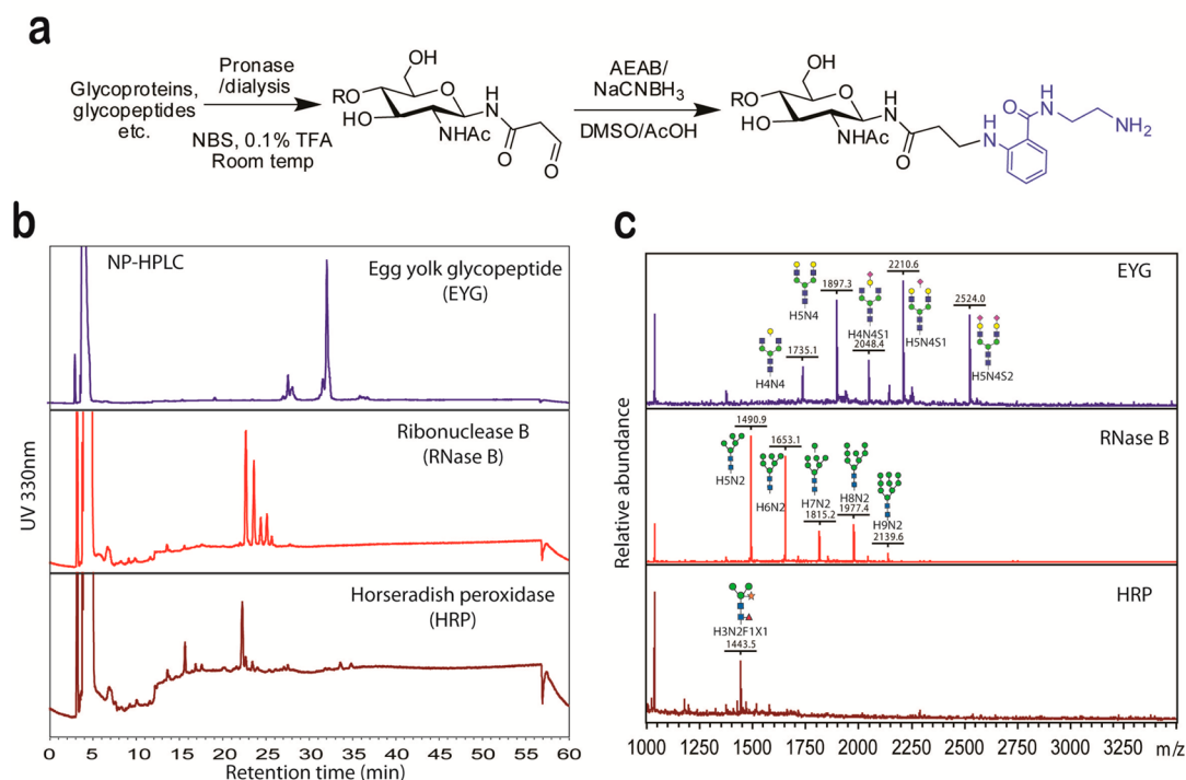
Figure 4. N-Glycan aldehyde can be prepared by NBS treatment of Pronase glycopeptides under acidic conditions and conjugated with AEAB. (a) Reaction scheme. (b) HPLC profiles. (c) MALDI-TOF MS of conjugates of glycan aldehyde with AEAB from egg yolk glycopeptide (top panels), ribonuclease B (middle panels), and horseradish peroxidase (bottom panels).
