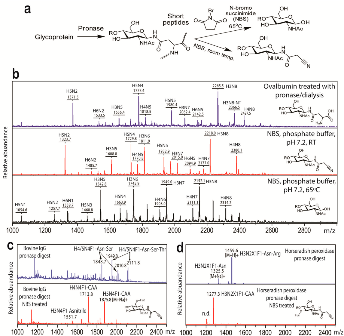
Figure 2. NBS treatment of Pronase digested glycopeptides generates glycan nitriles or reducing sugars. (a) Reaction scheme of Pronase digest and NBS treatment. (b) MALDI-TOF profiles of Pronase digested ovalbumin glycoamino acids (top panel), after NBS treatment under room temperature (middle panel) or 65 °C (bottom panel). (c,d) MALDI-TOF profiles of Pronase glycopeptides from bovine IgG (c) and horseradish peroxidase (d) before (top panels) and after (bottom panels) NBS treatment.
