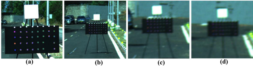
Fig. 6. The targeted scene at different distances (a: 5m, b: 25m, c: 50m, and d: 62m) from the hyperspectral imager.
