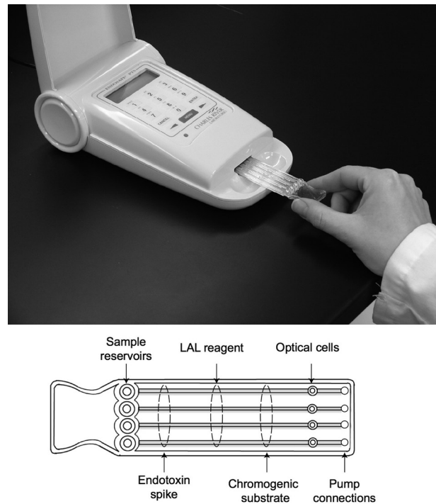
Fig.2. The limulus amoebocyte lysate (LAL) spectrophotometer (upper) and reagent cartridge (bottom) for the Endosafe ® PTS ™ system.
