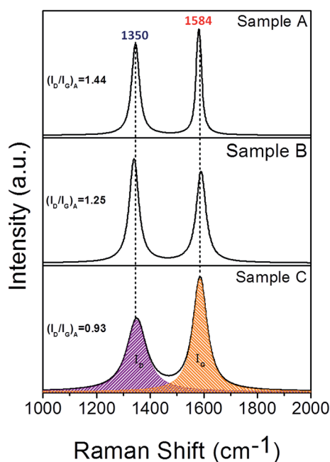
Fig. 4 Raman spectra of samples A, B and C synthesised under a mixed atmosphere of CH 4 and Ar with gas ratios of 1 : 8, 1 : 4 and 1 : 2, respectively.
