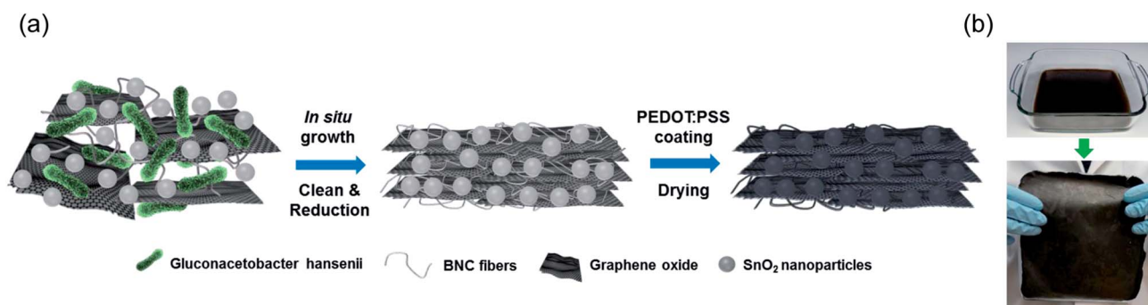
Fig. 1 (a) Schematic illustration showing the synthesis process of the PEDOT:PSS/SnO 2 /rGO/BNC electrode for supercapacitor. (b) Photographs of the SnO 2 /GO/BNC in hydrogel and dried states.
