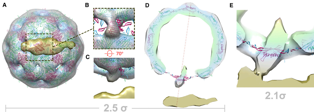
Figure 6. The MP Replaces a CP Dimer
