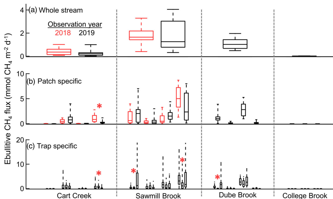
Fig. 2. Boxplots of observed ebullitive CH 4 fluxes at the scale of (a) the whole stream, (b) individual patches, and (c) individual traps with the 5 th and 95 th percentiles as the whisker extents. Red boxes represent fluxes from 2018 (only at Cart Creek and Sawmill Brook), while black boxes represent observations from 2019. Ebullitive fluxes at the trap scale (c) are shown for 2019 only. A single data point is the mean of all measured fluxes at the representative bubble traps for a 2-week period. Red asterisks mark comparisons where there is a significant difference in the mean ebullitive CH 4 flux between years (a and b) or traps (c) based on a Wilcoxon ranked sum or Kruskal–Wallis test, respectively.
