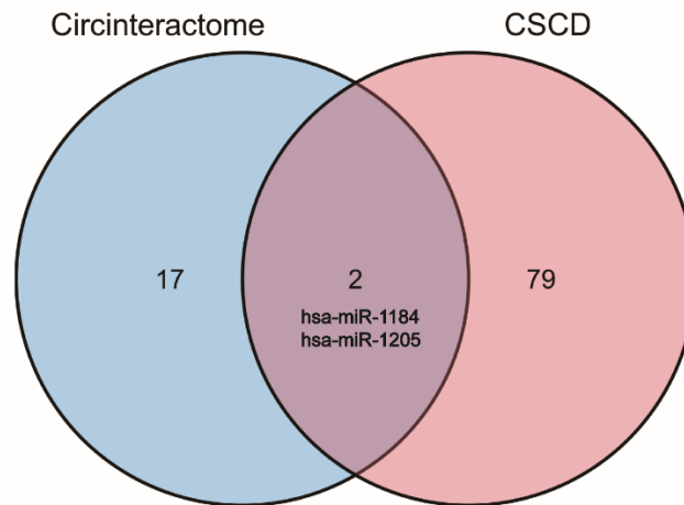
Supplementary Figure 3. The predicted miRNAs from CSCD and circinteractome databases were taken as intersection.
