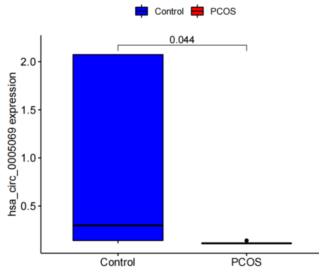
Supplementary Figure 2. Box plot of differential circRNA.
