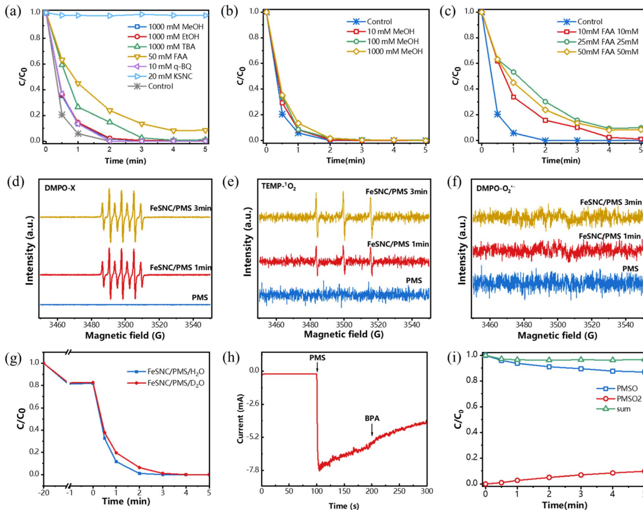
Fig. 5 (a–c) Impact of scavengers on BPA degradation in the FeSNC/PMS system; EPR analysis for DMPO-X (d), ^1O_2 (e), and O_2^{\bullet-} (f) detection of FeSNC/PMS system; (g) BPA degradation efficiency in different solvents; (h) amperometric I-t curves upon the addition of PMS and BPA; (i) PMSO loss and PMSO _2 production in the FeSNC/PMS system.
