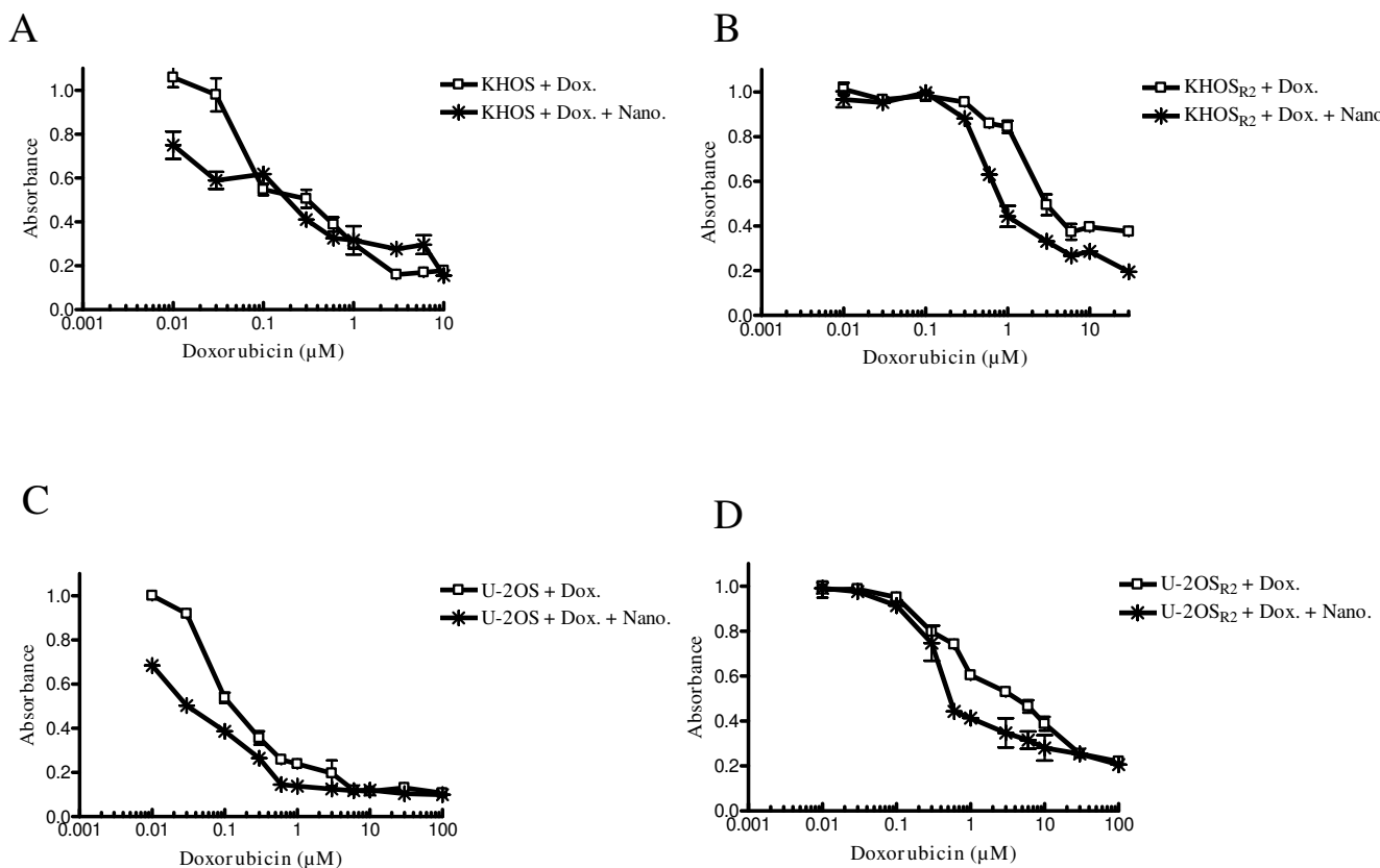
Figure 4 The effect of doxorubicin alone or nanoparticle loaded with doxorubicin on KHOS, KHOS R2 , U-2OS, and U-2OS R2 was analyzed (A-D). Varying concentrations of doxorubicin was added and consequently cultured for 5 days. Nanoparticle loaded with doxorubicin showed increased anti-proliferative activity in both drug sensitive and resistant osteosarcoma cell lines in a dose dependent manner. Growth inhibition was assessed by MTT as described under Methods. The experiment was repeated four times in triplicate.
