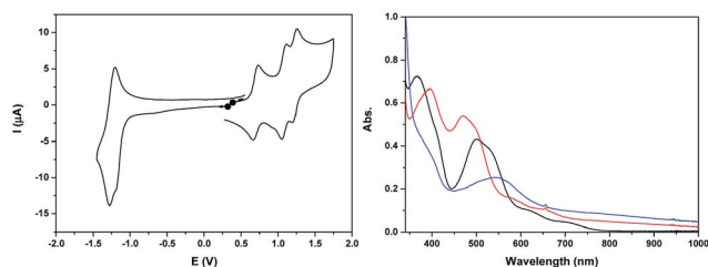
Fig. 2 (Left) Cyclic voltammogram of a 0.25 \text{ mM} solution of \text{Ru}_2\text{Co}-\text{OAc}_2 in 0.1 \text{ M} [(n\text{Bu}_4\text{N})\text{ClO}_4] in \text{CH}_3\text{CN} , at a scan rate of 100 \text{ mV s}^{-1} . (Right) UV-visible absorption spectra of a 0.25 \text{ mM} solution of \text{Ru}_2\text{Co}-\text{OAc}_2 in 0.1 \text{ M} [(n\text{Bu}_4\text{N})\text{ClO}_4] in \text{CH}_3\text{CN} , in oxidation states (black) \text{Ru}_2(\text{II})\text{Co}(\text{II}) , (red) \text{Ru}_2(\text{II})\text{Co}(\text{III}) and (blue) \text{Ru}_2(\text{III})\text{Co}(\text{III}) .
