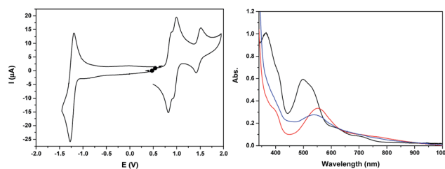
Fig. 3 (Left) Cyclic voltammogram of a 0.41 \text{ mM} solution of \text{Ru}_2\text{Mn}-\text{OAc}_2 in 0.1 \text{ M} [(n\text{Bu}_4\text{N})\text{ClO}_4] in \text{CH}_3\text{CN} , at a scan rate of 50 \text{ mV s}^{-1} . (Right) UV-visible absorption spectra of a 0.41 \text{ mM} solution of \text{Ru}_2\text{Mn}-\text{OAc}_2 in 0.1 \text{ M} [(n\text{Bu}_4\text{N})\text{ClO}_4] in \text{CH}_3\text{CN} , in oxidation states, (black) \text{Ru}_2(\text{II})\text{Mn}(\text{II}) , (red) \text{Ru}_2(\text{II})\text{Mn}(\text{III}) and (blue) \text{Ru}_2(\text{III})\text{Mn}(\text{III}) .
