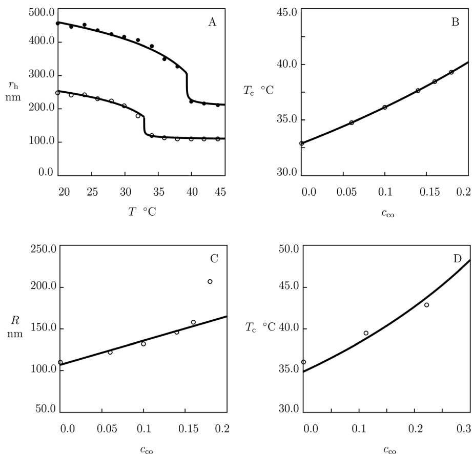
Fig. 6 (A) Hydrodynamic radius r_h of microgel particles versus temperature T . Symbols: experimental data 64 on P(NIPAm–DMAAm) microgels with molar fractions of comonomers c_{co} = 0 (O) and c_{co} = 0.18 (●). Solid lines: results of simulation. (B) Volume phase transition temperature T_c versus molar fraction of comonomers c_{co} . Circles: experimental data. Solid line: predictions of the model. (C) Radius R versus molar fraction of comonomers c_{co} . Circles: treatment of observations. Solid line: results of simulation. (D) Volume phase transition temperature T_c versus molar fraction of comonomers c_{co} . Circles: experimental data 57 on P(NIPAm–DMAAm) microgels. Solid line: predictions of the model.
