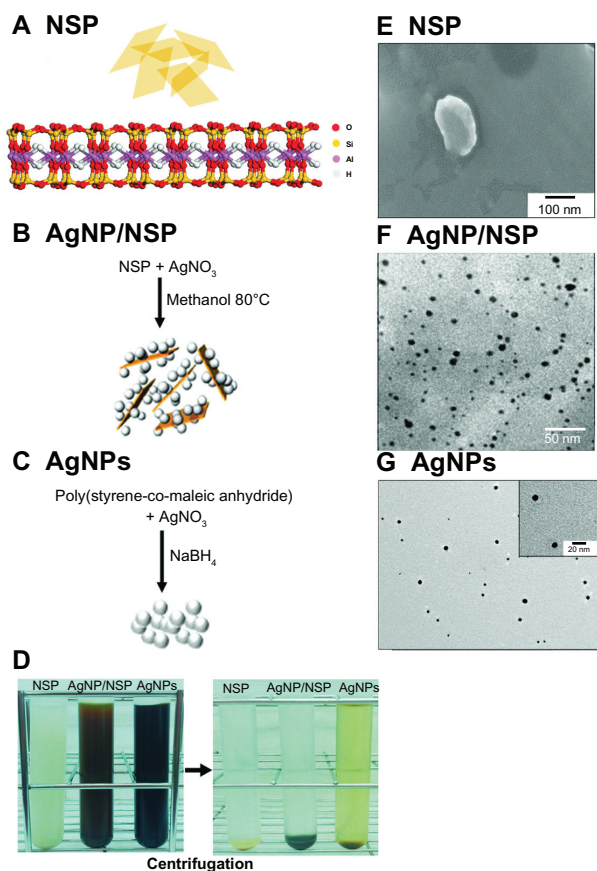
Figure 1 The characteristics of the nanoscale silicate platelet (NSP), silver nanoparticle (AgNP)/NSP, and AgNPs. (A–C) The molecular structure of NSP produced by ChemDraw is illustrated (A). The shapes and fabrication procedures of NSP (A), AgNP/NSP (B), and AgNPs (C) are illustrated. (D) The synthesized nanomaterials were precipitated by the centrifugation at 140,000 \times g for 20 hours at 20^\circ\text{C} . (E–G) Scanning electronic microscopy pictures of the NSP (E), AgNP/NSP, (F) and AgNPs (G) are presented.
