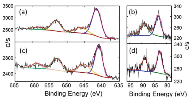
Fig. 4 High-resolution Mn 2p spectra of (a) \text{PhB}(\text{MesIm})_3\text{Mn}\equiv\text{N} ( 2 ) and (c) \text{PhB}(\text{MesIm})_3\text{MnCl} ( 1 ). The black line represents the experimental data, the red line shows the fit, and the blue and green lines represent Mn 2p_{3/2} and Mn 2p_{1/2} components, respectively, while the brown line represents shake-up satellites. See Table S3† for fitting parameters. High-resolution Mn 3s spectra of (b) \text{PhB}(\text{MesIm})_3\text{Mn}\equiv\text{N} ( 2 ) and (d) \text{PhB}(\text{MesIm})_3\text{MnCl} ( 1 ). The black line represents the experimental data, the red line shows fit, and the blue and green lines represent Mn 3s split components. See Table S4† for fitting parameters.
