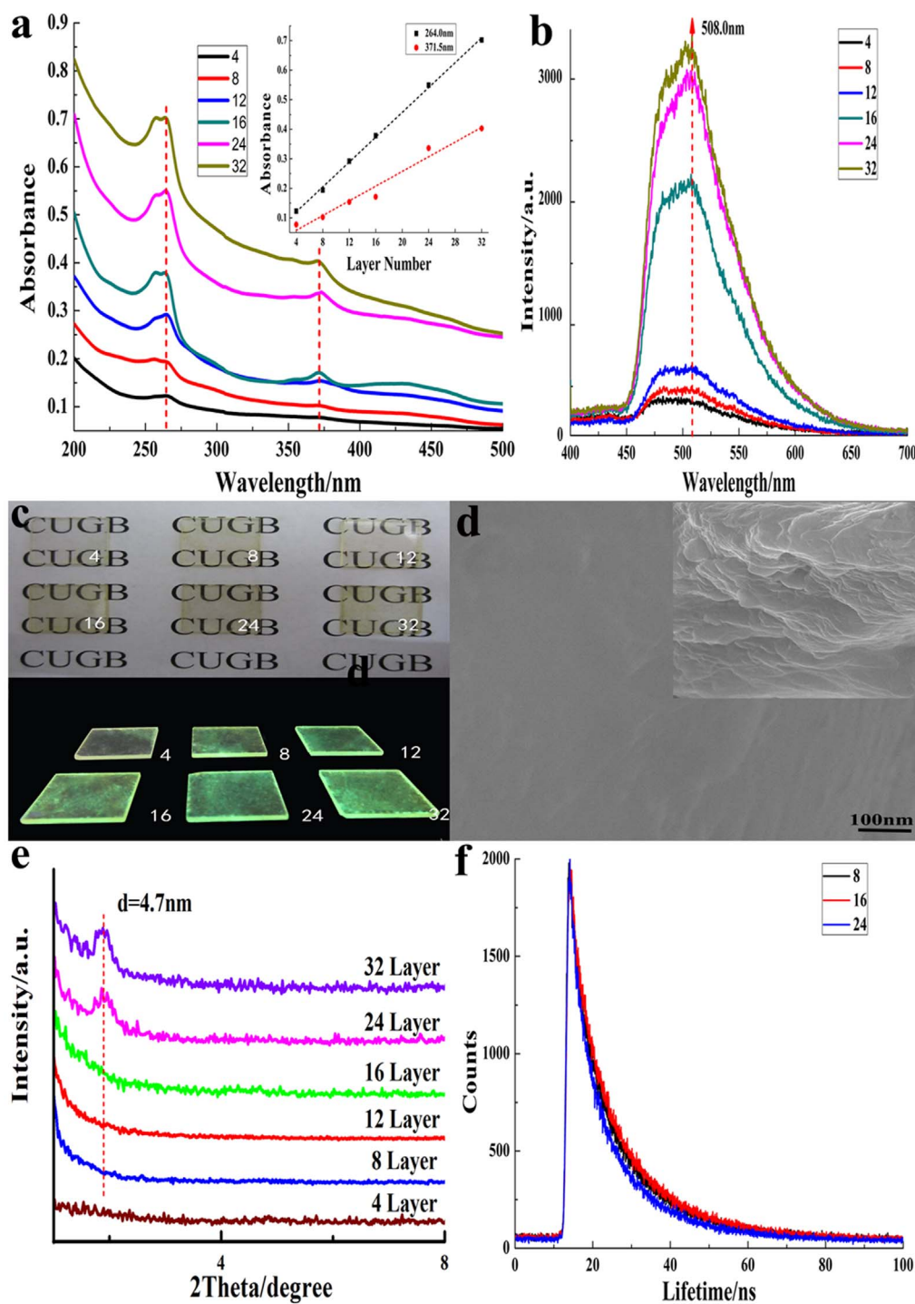
Figure 2 | Characterization of (\text{NiFe-LDHs}/\text{BNMA@PVA})_n OMFs (a) UV-visible absorption spectra, the inset shows the absorbance increasing linear relationship in 264.0 nm and 371.5 nm. (b) Photoluminescence spectra. (c) Photographs of OMFs with different bilayer numbers under daylight and UV light (365 nm), respectively. (d) The top view of the SEM image, the inset shows the side view of the SEM image. (e) Small angle XRD patterns. (f) Fluorescence decay profiles.
