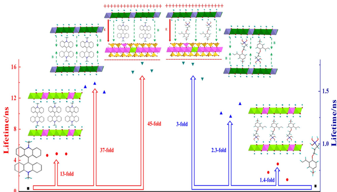
Figure 6 | The comparison of BNMA and APPV' lifetimes under the different environments. Black dots represent the luminescent lifetimes of pristine BNMA or APPV, the red stand for the lifetimes of (MgAl-LDHs/BNMA@PVS) n OMFs or (MgAl-LDHs/APPV) n OMFs, and the blue show the luminescent lifetimes of (NiFe-LDHs/BNMA@PVA) n OMFs or (NiFe-LDHs/APPV@PVA) n OMFs. The dark green stand for the luminescent lifetimes of (MMT/BNMA@PVA/NiFe-LDHs/BNMA@VA) n OMFs or (MMT/APPV@PVA/NiFe-LDHs/APPV@PVA) n OMFs.
