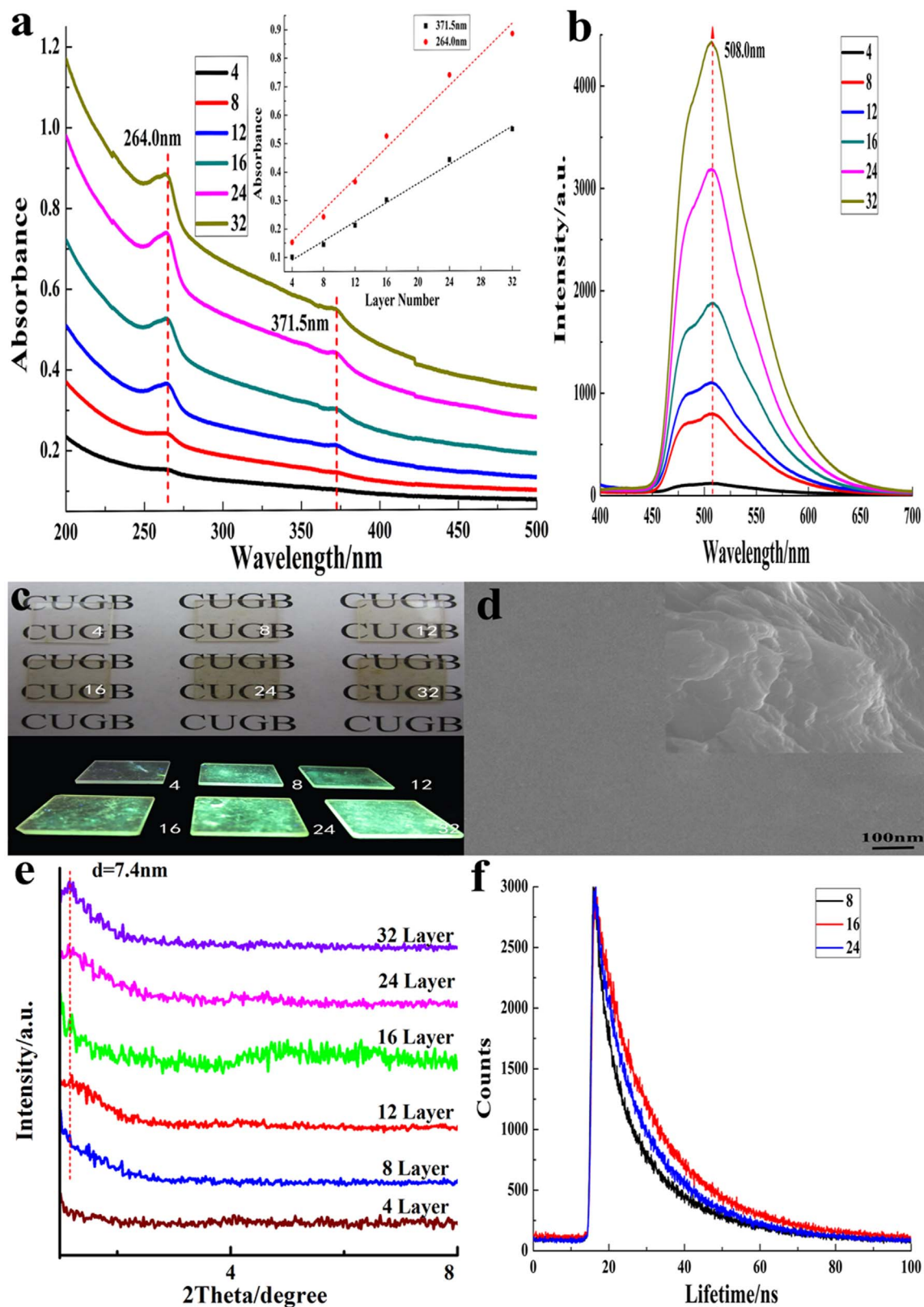
Figure 3 | Characterization of (\text{MMT}/\text{BNMA}@PVA/\text{NiFe-LDHs}/\text{BNMA}@PVA)_n OMFs (a) UV-visible absorption spectra, the inset shows the absorbance increasing linear relationship in 264.0 nm and 371.5 nm. (b) Photoluminescence spectra. (c) Photographs of OMFs with different bilayer numbers under daylight and UV light (365 nm), respectively. (d) The top view of the SEM image, the inset shows the side view of the SEM image. (e) Small angle XRD patterns. (f) Fluorescence decay profiles.
