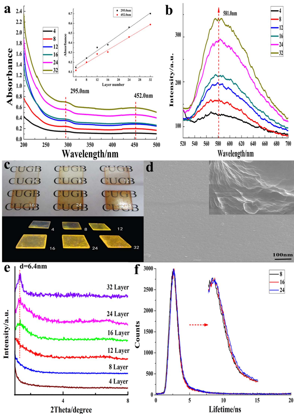
Figure 4 | Characterization of (\text{NiFe-LDHs}/\text{APPV@PVA})_n OMFs (a) UV-visible absorption spectra, the inset shows the absorbance increasing linear relationship in 295.0 nm and 452.0 nm. (b) Photoluminescence spectra. (c) Photographs of OMFs with different bilayer numbers under daylight and UV light (365 nm), respectively. (d) The top view of the SEM image, the inset shows the side view of the SEM image. (e) Small angle XRD patterns. (f) Fluorescence decay profiles.
