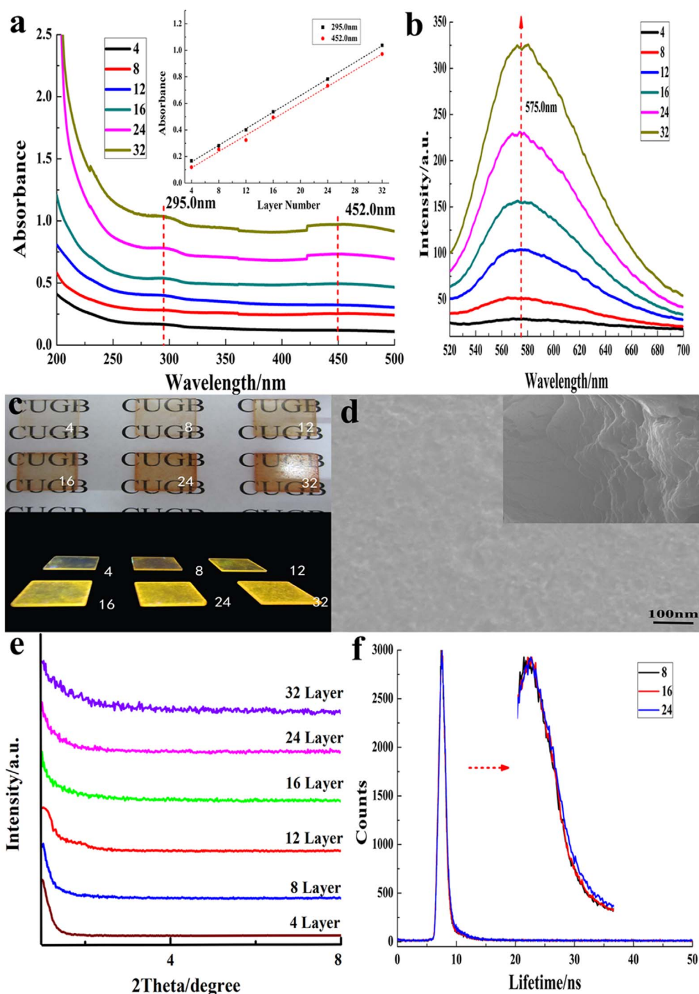
Figure 5 | Characterization of (\text{MMT}/\text{APPV}@PVA/\text{NiFe-LDHs}/\text{APPV}@PVA)_n OMFs (a) UV-visible absorption spectra, the inset shows the absorbance increasing linear relationship in 295.0 nm and 452.0 nm. (b) Photoluminescence spectra. (c) Photographs of OMFs with different bilayer numbers under daylight and UV light (365 nm), respectively. (d) The top view of the SEM image, the inset shows the side view of the SEM image. (e) Small angle XRD patterns. (f) Fluorescence decay profiles.
