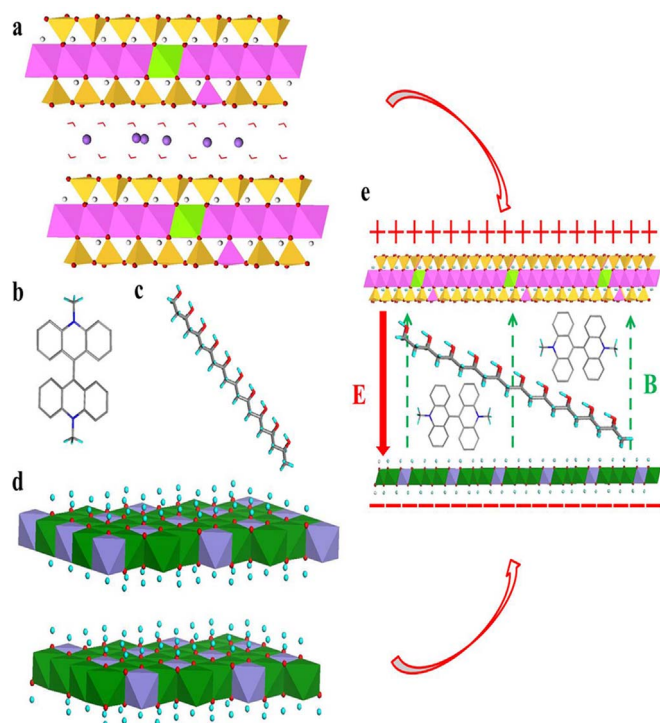
Figure 1 | (a) A representation of MMT, (b) Structure of APPV (c) Structure of PVA Chemical formula of APPV, (d) A representation of NiFe-LDHs, (e) The assembly of OMFs with the PEM and FME. pink: aluminum element, green: magnesium element, yellow: silicon element, dark green: nickel element, purple: iron element.
