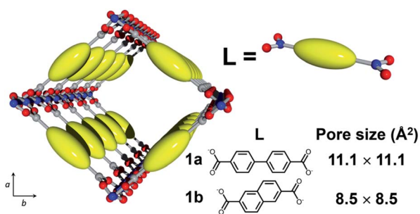
Fig. 2 Schematic image for the crystal structure of 1 (Al, blue; O, red; C, gray; 1a , L = 4,4'-biphenyldicarboxylate; 1b , L = 2,6-naphthalenedicarboxylate).
