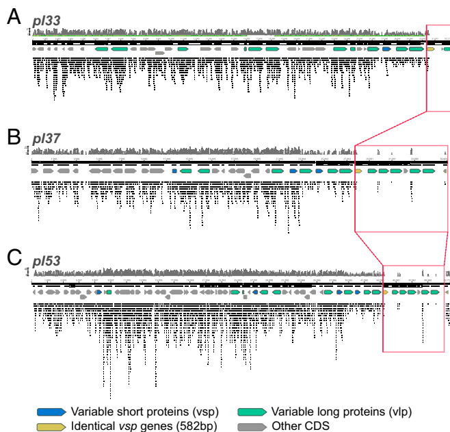
Fig. 3. Alignment of OSL9A-B reads to B. recurrentis plasmids p133 (A), p137 (B), and p153 (C). Across all plasmids a section at the 3' end of the linear plasmids is missing starting with 80% of a vsp gene. The regions boxed in red share identities of 99–100%. Tiled reads seen within the boxed regions are nonunique reads mapping to sequences conserved across multiple plasmids.
