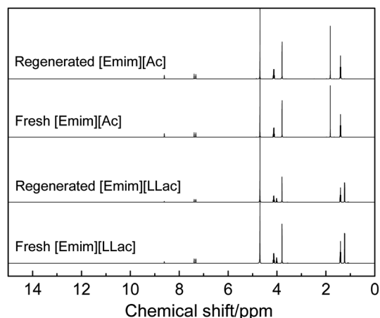
Fig. 11 ^1\text{H} NMR spectra of the fresh and regenerated HFILs. Conditions: initial phenol content, 103.215 \text{ g dm}^{-3} ; separation agents, [Emim][LLac] and [Emim][Ac]; solvent, \text{D}_2\text{O} ; mass, about 20 \text{ mg} ; sampling frequency, 16 .
