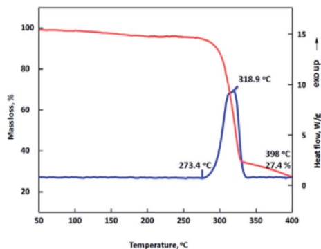
Fig. 2 DSC-TG trace of MDO under a heating rate of 10\text{ }^{\circ}\text{C min}^{-1} .
