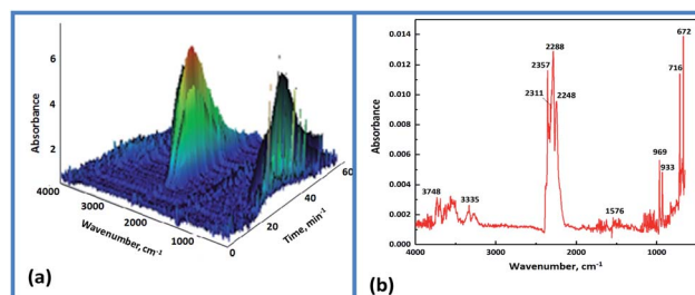
Fig. 4 (a) 3D IR absorption spectrum of MDO at a heating rate of 10\text{ }^{\circ}\text{C min}^{-1} ; (b) IR spectrum of MDO at 319\text{ }^{\circ}\text{C} .
