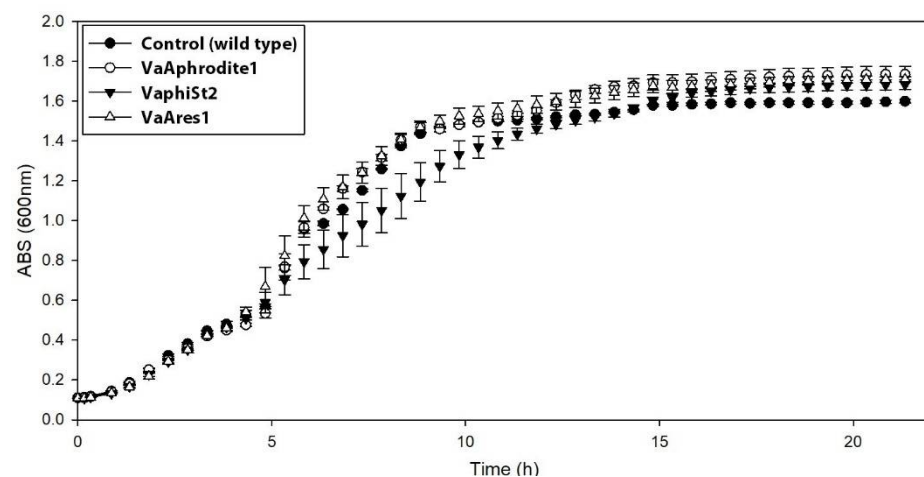
Figure 1. Growth kinetics of phage-resistant and phage-susceptible strains. Growth (average, \pm SE) of the Control (phage-susceptible strains; black circle; n = 3 ), VaAphrodite1 strains (phage strains resistant to bacteriophage Aphrodite1; white circle; n = 9 ), VaphiSt2 strains (phage strains resistant to bacteriophage phiSt2; black triangle; n = 9 ), and VaAres1 strains (phage strains resistant to bacteriophage Ares1; white triangle; n = 9 ).
