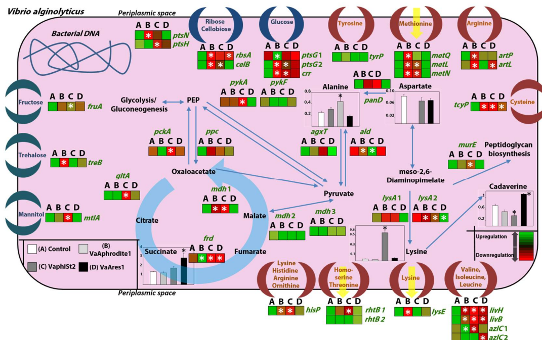
Figure 6. Schematic representation of metabolic reprogramming that takes place in phage-resistant strains. Relative transcript levels (heat maps) of sugar–polyol transporters (blue crescent moon) and amino acid transporters (brown crescent moon) of the inner bacterial membrane, accompanied by genes that are involved in important biochemical intracellular pathways of phage-susceptible (A) and phage-resistant (B, C, D) strains. Bars represent relative content levels of intracellular metabolites ( \pm SE) in susceptible (white) and resistant strains in bacteriophages Aphrodite1 (light grey), phiSt2 (dark grey), and Ares1 (black). Blue arrows represent biochemical pathways in brief; the light blue round arrow represents part of the TCA cycle; yellow arrows represent putative extraction of metabolites through membrane proteins. White and black asterisks represent statistically significant differences between phage-susceptible strains and phage-resistant strains (ANOVA, post-hoc analysis Student's t -test, p < 0.05 ).
