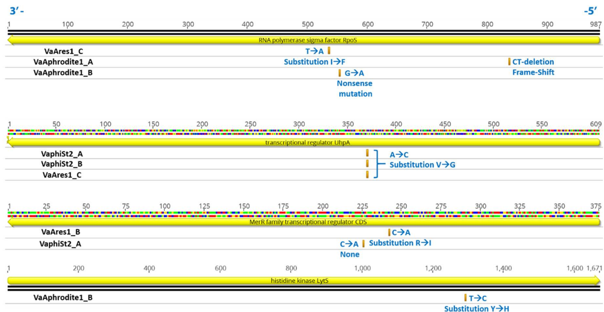
Figure 5. Schematic representation of nucleotide sequences of four CDSs and their orientation, involved in transcriptional regulation of V. alginolyticus , and their SNPs as presented in the text. Yellow represents CDS; orange, SNP positions; and blue, information of SNPs and protein effects in resistant bacteria VaAphrodite1 (A, B), VaphiSt2 (A, B), and VaAres1 (B, C). Orientation of the genome is also shown with blue numbers.
