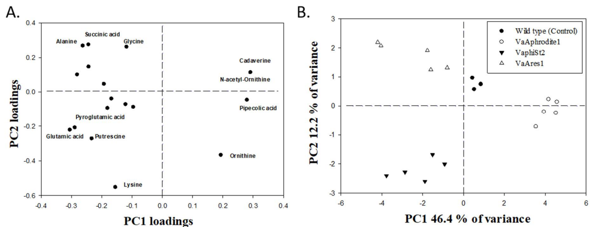
Figure 4. Partial Least Squares Discriminant Analysis (PLS-DA) of metabolomics results. and representation of component 1 (46.4%) and component 2 (12.2%) (A) of the identified metabolites discussed in the results and discussion section comparing the wild type (Control, phage-susceptible strains; n = 4 ), VaAphrodite1 strains (phage strains resistant to bacteriophage Aphrodite1; n = 5 ), VaphiSt2 strains (phage strains resistant to bacteriophage phiSt2; n = 5 ), and VaAres1 strains (phage strains resistant to bacteriophage Ares1; n = 5 ). (B) Loadings of individually identified components showing the highest variability under the studied experimental conditions.
