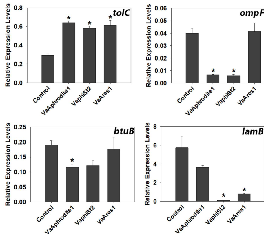
Figure 3. Relative expression levels of genes encoding for outer membrane and transmembrane proteins. Bars represent means \pm SE of independent biological repeats ( n = 3 ). Asterisks * indicate significantly different values based on Student's t -test. Statistical significance was postulated for p \leq 0.05 .
