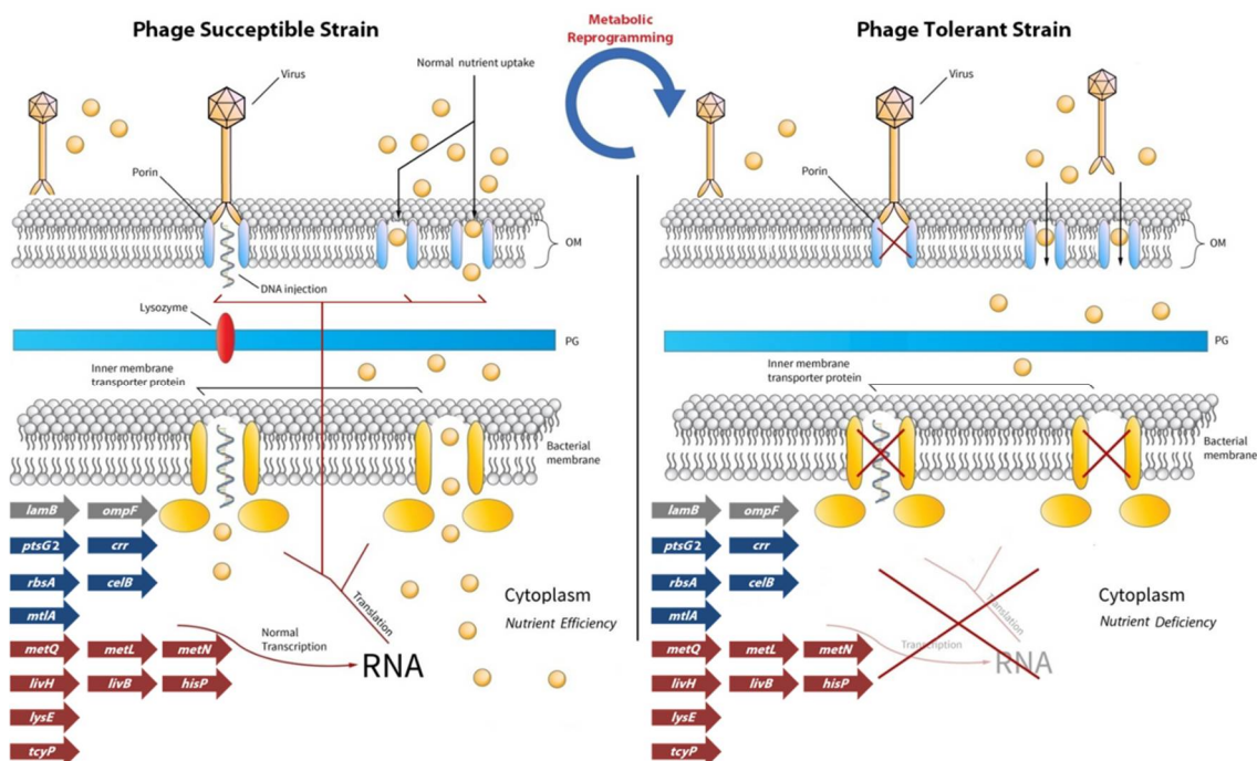
Figure 7. Schematic representation of how metabolic reprogramming of bacterial cells could introduce phage resistance against lytic bacteriophages after phage–host interaction. Arrows represent genes (as seen in Table 3) involved in nutrient assimilation or exportation for which their relative transcript levels were significantly downregulated compared to the control (wild-type) strains in the current study. Gray: outer membrane receptors ( lamB and ompF ); Blue: inner bacterial membrane sugars and polyols ( ptsG 2 , crr , rbsA , celB , mtlA ); Red: inner bacterial membrane amino acids ( metQ , metL , metN , livH , livB and hisP ). OM: outer membrane; PG: peptidoglycan layer.
