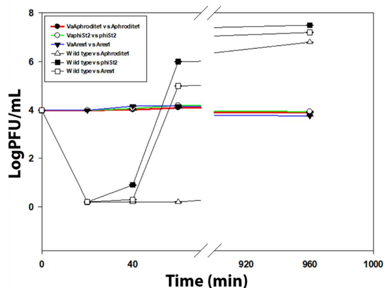
Figure 2. Adsorption assay for bacteriophages Aphrodite1, phiSt2, and Ares1 against their corresponding resistant strains. Initial titer was 10^4 , and cultures upon infection were in their exponential phase ( \pm SE; n = 3 ).
