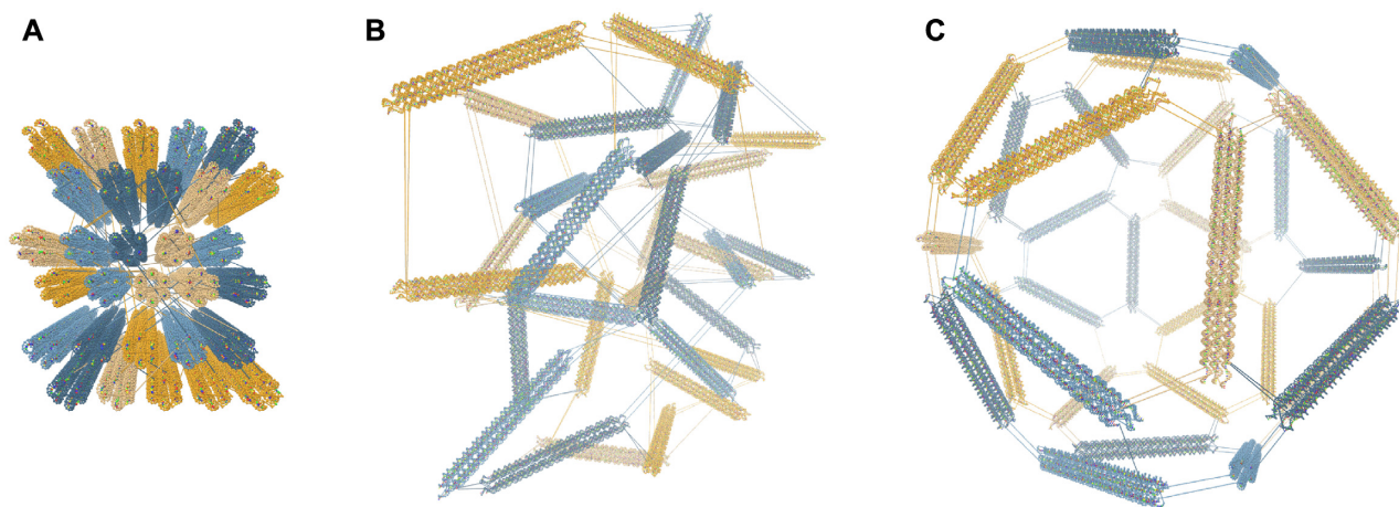
Figure 3. Rigid-body dynamics of clusters. Snapshots from the automatic rigid-body relaxation of an icosahedron, starting with the configuration converted from caDNAo (A), through the intermediate (B) where the dynamics are applied, and (C) the final resulting relaxed state.
