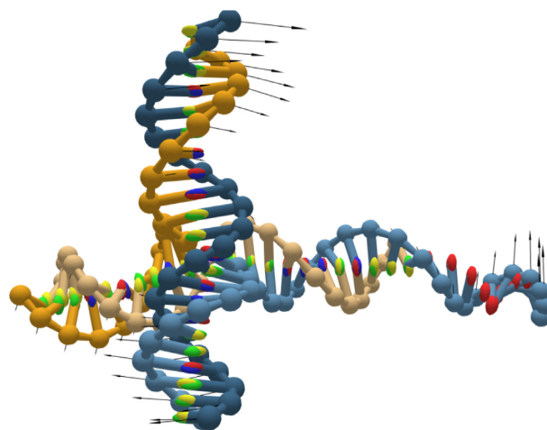
Figure 8. Principal component analysis of a Holliday junction visualized on oxView. Shown here is the top mode, which corresponds to a scissoring motion in the junction, with the arm ends having significantly higher average displacement than the crossover point.
