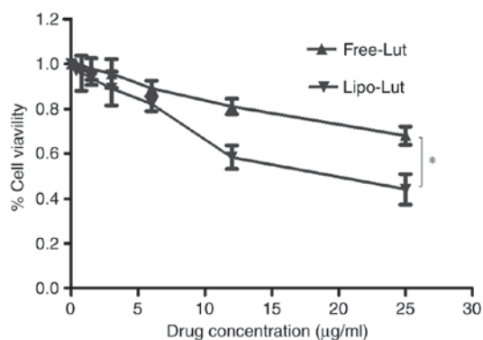
Figure 3. The effect of liposomal luteolin in CT26 cells viability. The CT26 cells were treated with different concentrations of Free-Lut or Lipo-Lut ( \mu\text{g/ml} ) for 24 h. After this treatment, the cell viability was measured by MTT assay. The data are expressed as the mean \pm standard deviation of three independent experiments. * P < 0.05 .
