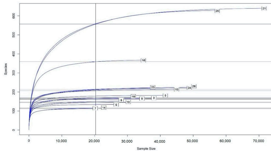
Figure 2. Rarefaction curve for sequence analysis of caecotrophs. The vertical axis shows the number of different species (operational taxonomic units, OTUs) that would be expected to be found after sampling the number of sequences shown on the horizontal axis. The curvature towards the horizontal indicates the greater sequencing effort required to observe new species. The curve was obtained with the Rarefaction Species Richness script from the Vegan package on the RStudio platform [15]. Group identification: T1 (healthy rabbits on a diet with 32% NDF): 3, 5, 6, and 7. T2 (healthy rabbits on a diet with 32% NDF): 8, 9, 10, and 14. T3 (rabbits that had ERE at the outset on a diet with 32% NDF): 15, 18, 19, and 20. T4 (rabbits that had ERE at the outset on a diet with 36% NDF): 21, 23, 24, and 26.
