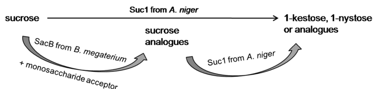
Figure 1 Enzymatic synthesis of novel oligofructosides. Oligofructosides used in this study were synthesized by the concerted action of two fructosyltransferases from B. megaterium (SacB) and A. niger (Suc1).
