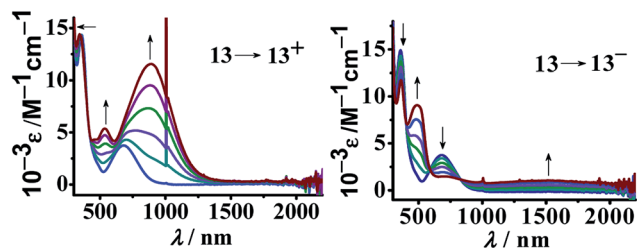
Fig. 15 UV-vis-NIR spectroelectrochemistry of 13^n in \text{CH}_3\text{CN} .
