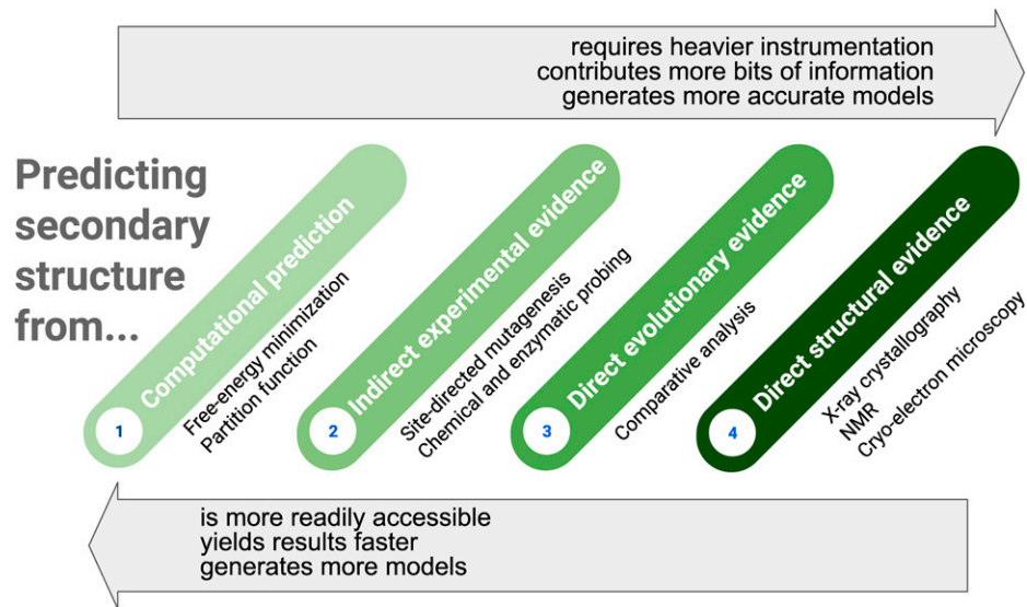
Fig. 6. Hierarchy in the methods commonly used to predict the secondary structure of an RNA. The confidence level in an RNA secondary structure model depends on the number of pieces of computational and experimental information used to predict that model (roughly increasing from left to right), which relates to the time to obtain that model (also increasing from left to right), which in turn is linked to accessibility to advanced instrumentation and expertise in structure determination methods.
