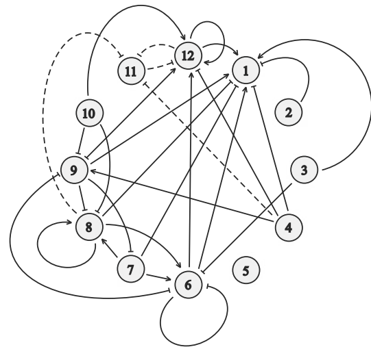
Fig. 4 A plausible gene cluster network in the lactose phase based on our criteria. The full lines correspond to the \kappa_{q}^p ’s of Eq. 22 while the dashed lines represent the \alpha_{q}^p ’s and \beta_{q}^p ’s in Eq. 21
