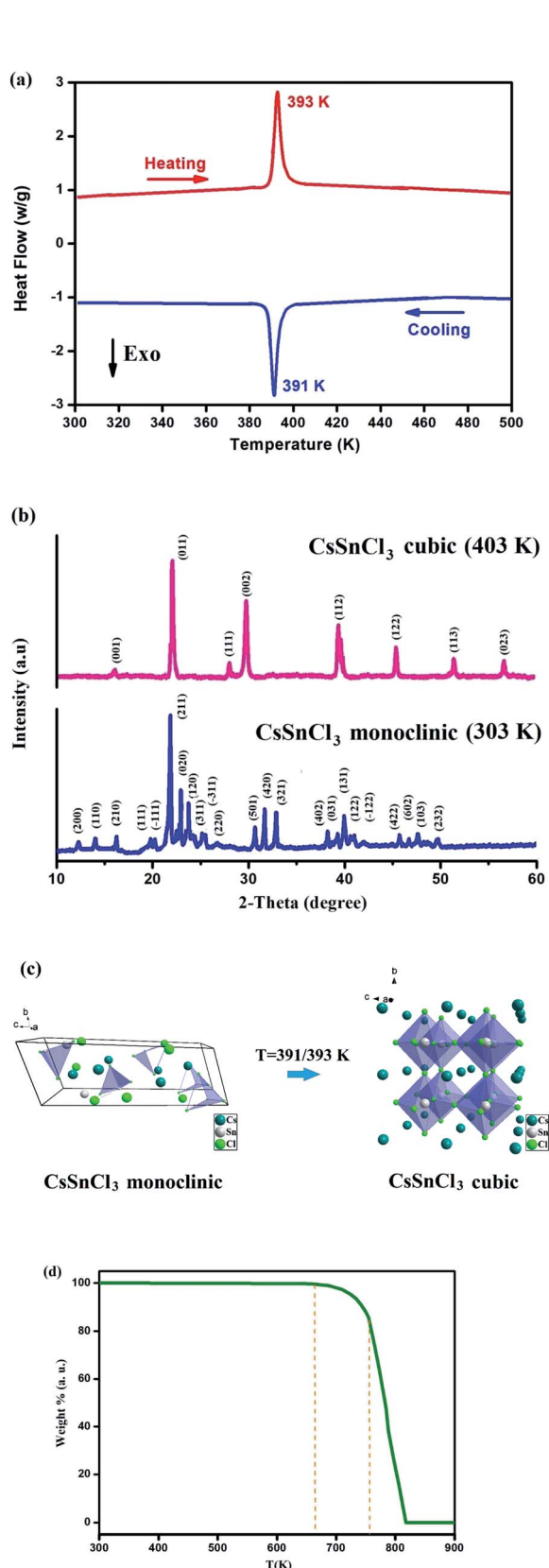
Fig. 1 (a) DSC curves of CsSnCl 3 . (b) PXRD patterns of CsSnCl 3 at 303 and 403 K. (c) Constructed monoclinic and cubic structures of CsSnCl 3 . The crystal structures were designed using VESTA. (d) TG curve of CsSnCl 3 in the temperature range of 300–900 K.
