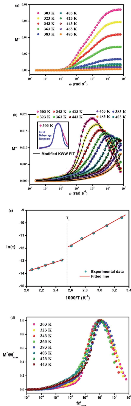
Fig. 6 (a) Frequency dependence of the real part of electric modulus of CsSnCl 3 . (b) Frequency dependence of the imaginary part of the electric modulus of the sample. Inset of (b) deviation from the ideal Debye response at 303 K. (c) Arrhenius plot of the maximum frequency of M''(\omega) of the sample. (d) Normalized imaginary electric modulus M''/M''_{\max} vs. f/f_{\max} at different temperatures.
