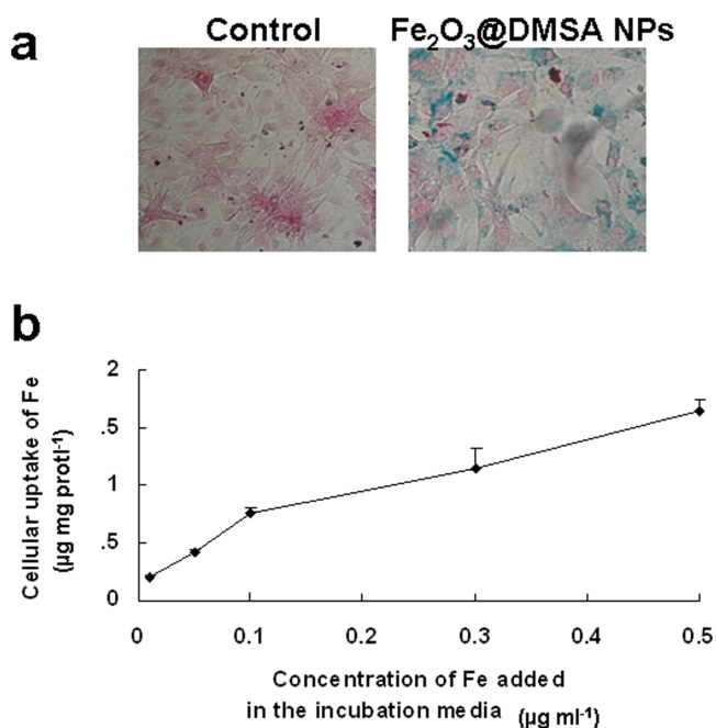
Figure 3 | The uptake of \text{Fe}_2\text{O}_3 @DMSA NPs by cardiomyocytes. (a) Prussian blue staining of cardiomyocytes incubated without (control) and with 0.1 \text{ mg ml}^{-1} of \text{Fe}_2\text{O}_3 @DMSA NPs. (b) The uptake of \text{Fe}_2\text{O}_3 @DMSA NPs at different doses ( n = 6 ).
