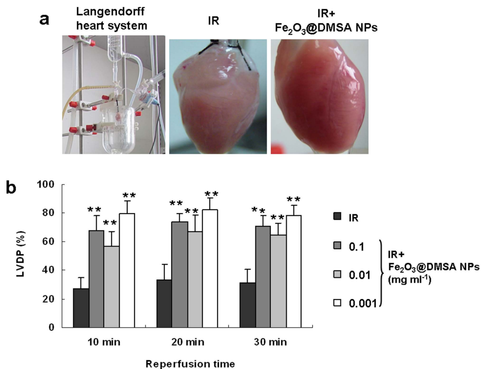
Figure 2 | \text{Fe}_2\text{O}_3 @DMSA NPs have a cardiprotective activity in guinea pig Langendorff heart following 30 min of ischemia and 30 min of reperfusion (IR). (a) The Langendorff heart system (left), a heart perfused without (IR, middle) and with 0.001 \text{ mg ml}^{-1} of \text{Fe}_2\text{O}_3 @DMSA NPs (IR + \text{Fe}_2\text{O}_3 @DMSA NPs, right) after ischemia. (b) LVDPs were recorded with perfused hearts without and with 0.1 , 0.01 and 0.001 \text{ mg ml}^{-1} of \text{Fe}_2\text{O}_3 @DMSA NPs at 10, 20 and 30 min after perfusion. ** p < 0.01 vs the IR group; n = 6 .
