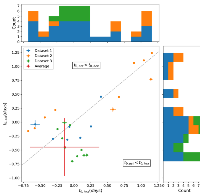
Figure 4. Resulting fit parameters for three repeats, with 10 aliquots each, of the emergence experiments described in Figure 2. X axis depicts nucleation time of the hexamer replicators, Y axis of the octamer replicators. If a data point is found above the diagonal (dashed line) hexamers nucleated before octamers, and vice versa, showing the spread in nucleation times. Error bars indicate standard deviations in the fitting parameters, but these are too small to be observed for most points ( R^2 = 0.933 ). The weighted average nucleation time is indicated in red, showing that on average, octamers nucleate before hexamers. This observation is consistent with the fact that octamers are the dominant species in the majority of the samples. Above the axes, histograms of the found nucleation times are plotted.
