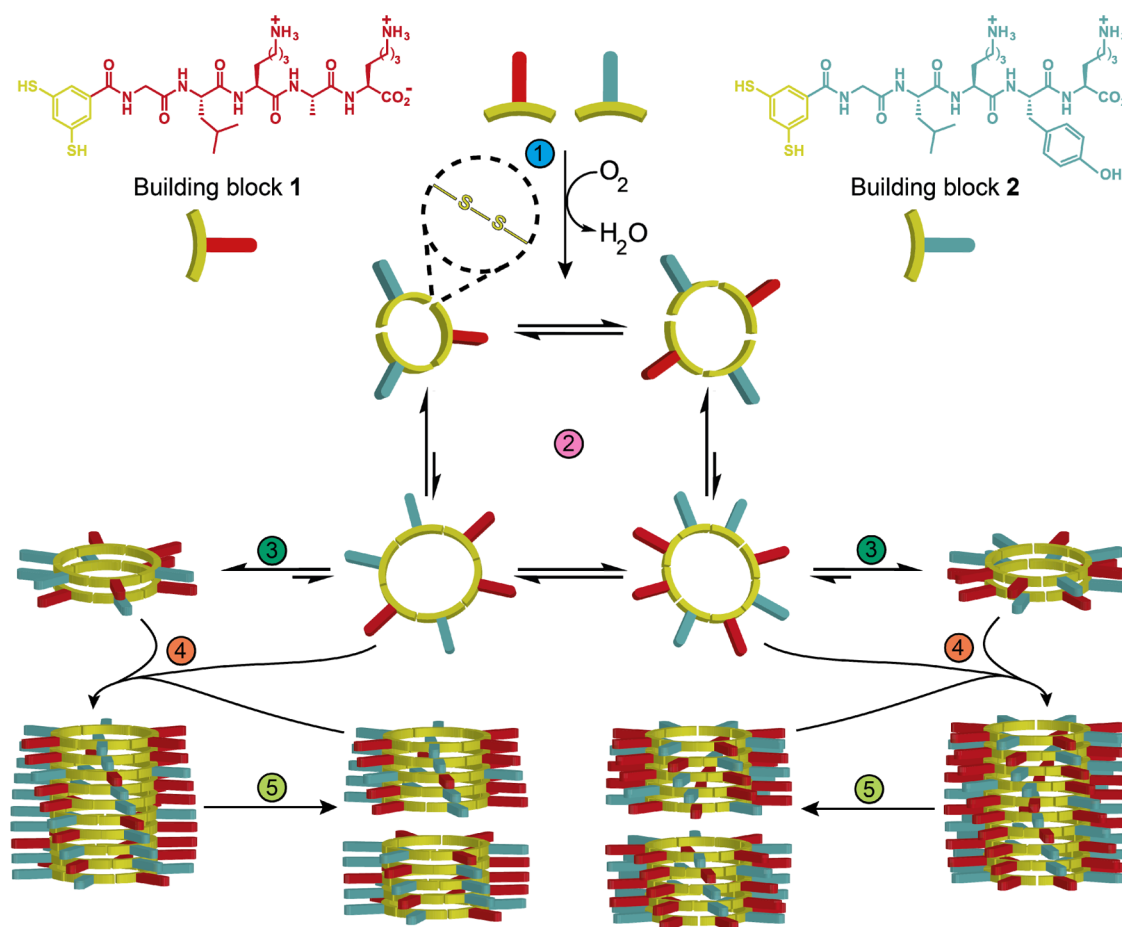
Figure 1. Molecular structures of building blocks 1 and 2 and schematic representation of the self-replication mechanism. Dithiol-building blocks, 1 and 2, are oxidized (1) to form a mixture of macrocycles with various ring sizes (2) that interconvert using thiol–disulfide chemistry. Two different nucleation steps can occur (3), leading to the formation of stacks of macrocycles containing six or eight monomer units. Both nuclei can elongate (4) to form fibers by consuming smaller macrocycles from the solution. Fragmentation of the fibers by mechanical agitation when the stack is sufficiently long (5) leads to an elongation/fragmentation regime, enabling exponential growth.
