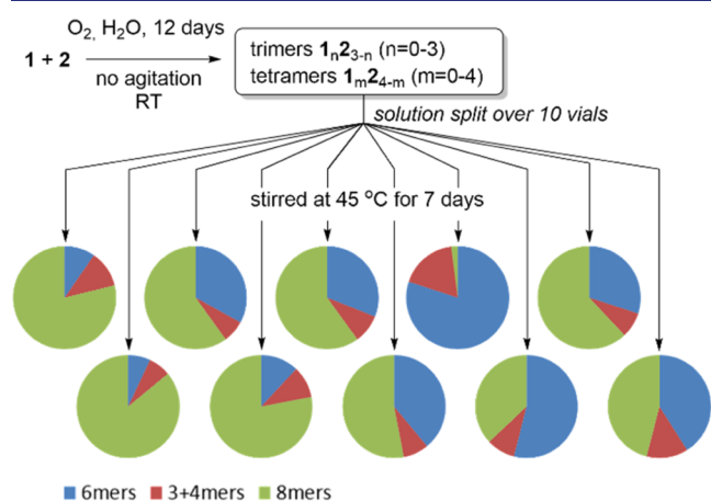
Figure 2. Final compositions of a DCL made from equimolar amounts of 1 and 2 , split into 10 smaller aliquots. Different outcomes with different ratios between hexamer, octamer, and trimer + tetramer were found.
