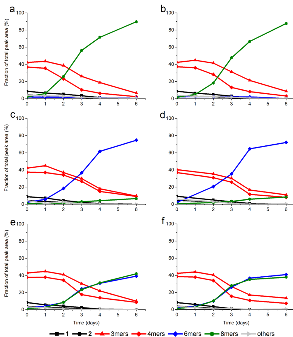
Figure 3. Kinetic traces of DCLs seeded with preformed self-replicators. (a, b) Seeded with 10 mol % preformed mixed octamer, (c, d) seeded with 10 mol % preformed mixed hexamer, and (e, f) seeded with 5 mol % of preformed mixed hexamer as well as 5 mol % preformed mixed octamer.
