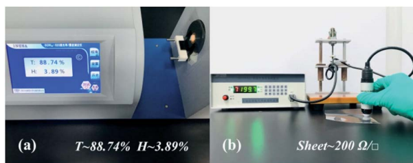
Fig. 6 Optoelectronic performances of flexible TCFs based on the ultra-long AgNWs including (a) transmittance and haze, and (b) sheet resistance.
