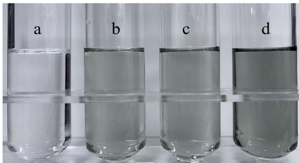
Figure 2 Visual inspection (color changes) of combinations of etoposide + ilaprazole sodium. (a) Negative control, etoposide + ilaprazole sodium in NS at 0 h; (b) Combination of etoposide + ilaprazole sodium in NS at 10 min, the color changed to light green; (c) Combination of etoposide + ilaprazole sodium in NS at 1 h, the color changed to blue-green; (d) Combination of etoposide + ilaprazole sodium in NS at 4 h; the color changed to dark green.
