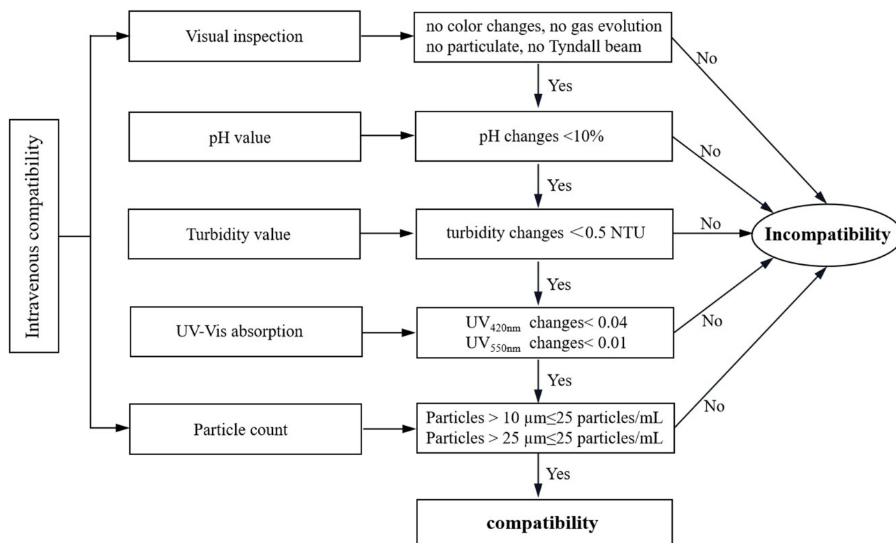
Figure 1 Diagram of compatibility justification.
