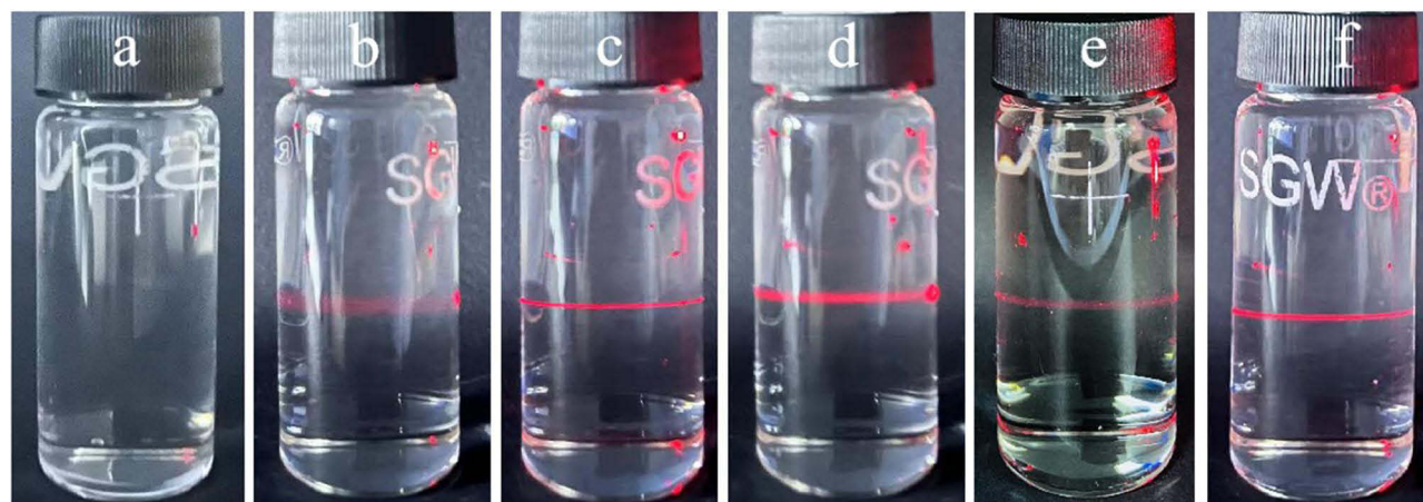
Figure 3 Tyndall beam of solutions. (a) Negative control, etoposide in NS; (b) Combination of etoposide + ceftazidime in NS at 4 h; (c) Combination of etoposide + cefuroxime sodium in NS at 1 h; (d) Combination of etoposide + glutathione in NS at 0 h; (e) Combination of etoposide + ilaprazole sodium in NS at 1 h; (f) Combination of etoposide + mycophenolate in D5W at 1 h.
