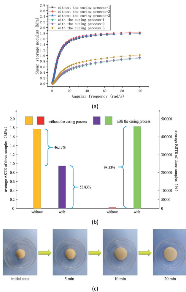
Fig. 3 (a) The shear storage modulus of the continuously changing angular frequency from 0.1–100 \text{rad s}^{-1} ; (b) the average ASTE and RSTE of three samples and the change rules and (c) the relaxation of the sample in a natural state.
