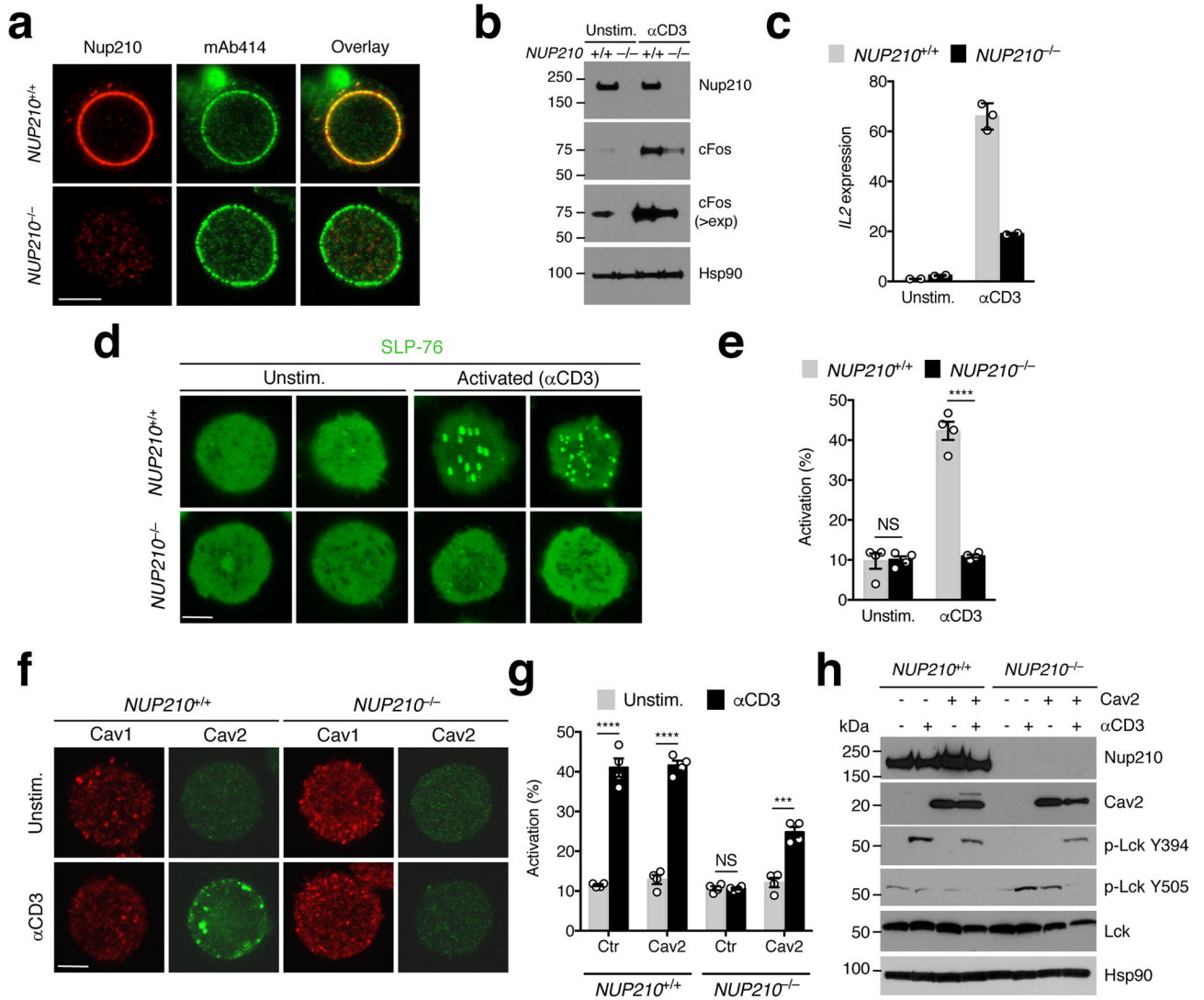
Fig. 7. Nup210 is required for the TCR-dependent induction of Cav2 expression (a) Immunofluorescence analysis of Nup210 and mAb414 in NUP210 +/+ or NUP210 -/- J14 SLP-76-EYFP cells. (b) Immunoblot analysis of Nup210 and cFos in resting and soluble anti-CD3-activated NUP210 +/+ or NUP210 -/- J14 SLP-76-EYFP cells. Hsp90 was used as loading control (>exp: higher exposure). (c) qPCR analysis of Il2 mRNA levels in resting or soluble anti-CD3-activated NUP210 +/+ or NUP210 -/- J14 SLP-76-EYFP cells. Il2 expression was normalized to Hprt1 . (d) Immunofluorescence analysis of SLP-76 clustering on the surface of unstimulated or anti-CD3-activated NUP210 +/+ or NUP210 -/- J14 SLP-76-EYFP cells. (e) The percentage of cells with SLP-76 foci from (d) was quantified. (f) Immunofluorescence analysis of Cav1 and Cav2 in unstimulated or anti-CD3-activated NUP210 +/+ or NUP210 -/- J14 SLP-76-EYFP cells. (g) The percentage of activated (SLP-76 cluster-positive cells) NUP210 +/+ or NUP210 -/- J14 SLP-76-EYFP cells expressing control (empty vector) or Cav2 was quantified after stimulation with soluble anti-CD3. (h) Immunoblot analysis of Nup210, Cav2, p-Lck Y394, p-Lck Y505, and total Lck in unstimulated or anti-CD3-activated NUP210 +/+ or NUP210 -/- J14 SLP-76-EYFP cells
