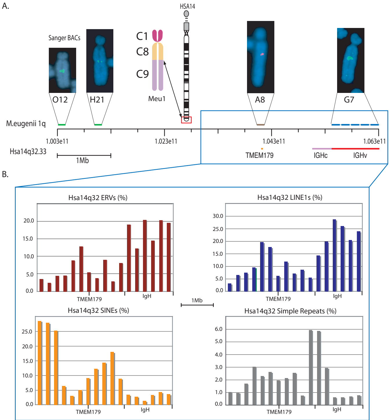
Figure 7 Map of Hsa14q32 and Meu Iq. (A) Map of M. eugenii Iq compared to the orthologous human 14q32.33 showing tammar BACs FISH mapped to the EB region of Iq and their relative position on I4q. BACs O12 and H21 have been identified by the Sanger Institute to be orthologous to Hsa14q32. BAC A8 and G7 were identified by screening the M. eugenii BAC library with KERV. BAC A8 contains a predicted protein with high homology to human TMEM179. BAC G7 contains regions with high identity to the entire region of the human immunoglobulin heavy chain variable region (IGHv). (B) The density of ERVs, LINE1s, SINEs, and simple repeats in the most distal 3.4 Mb of I4q32 in increments of 200 kb, including the IGH region and TMEM179.
